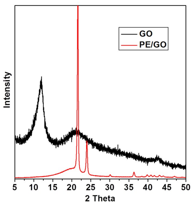
Figure S1. XRD patterns of GO and PE/GO
