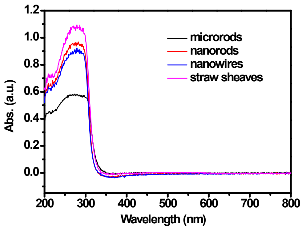
Fig. S1 The UV-vis diffuse reflectance spectra of Bi(C 2 O 4 )OH samples
