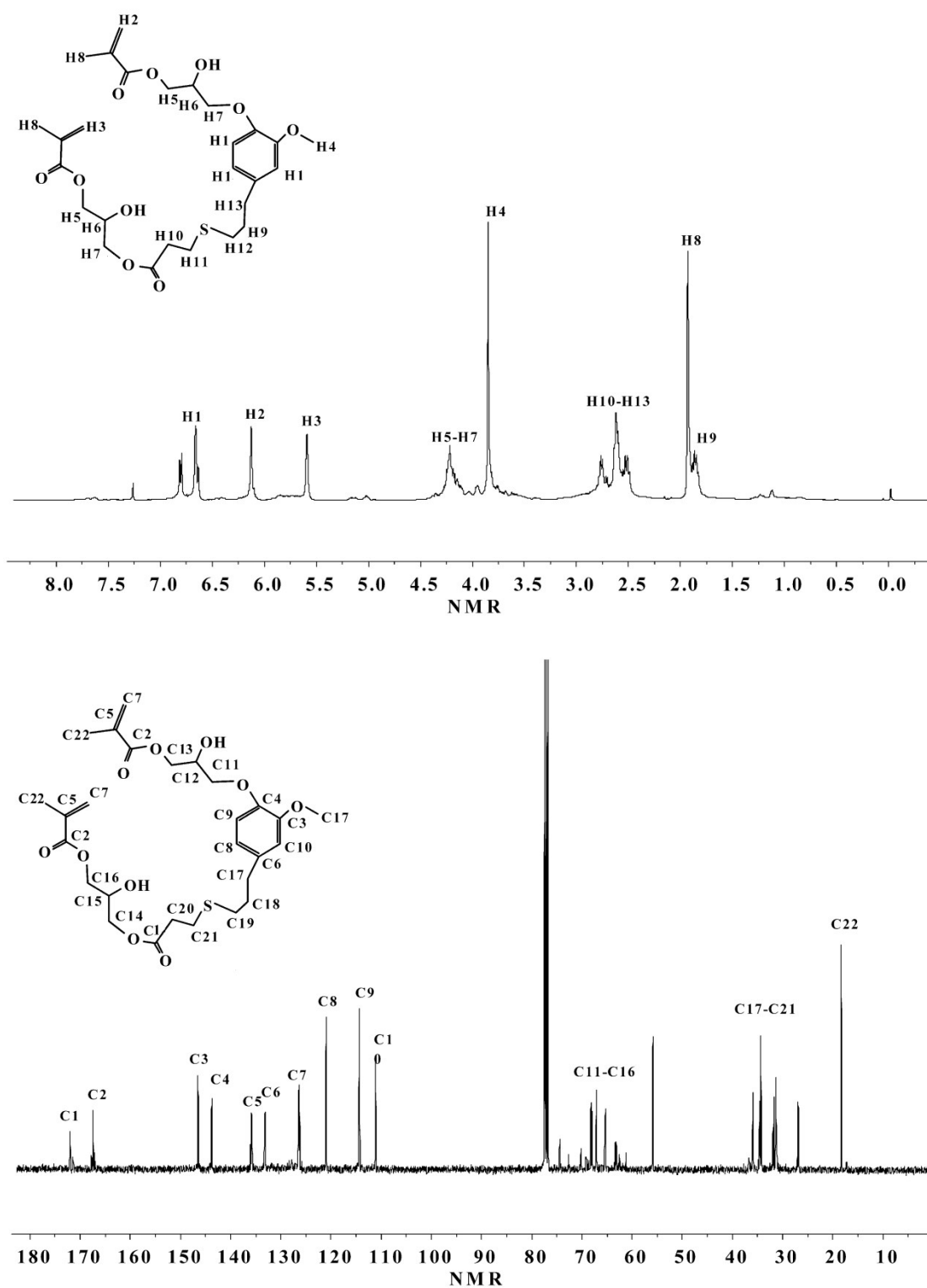
Fig. 4 The ^1\text{H} NMR and ^{13}\text{C} NMR spectra of EM2G.
