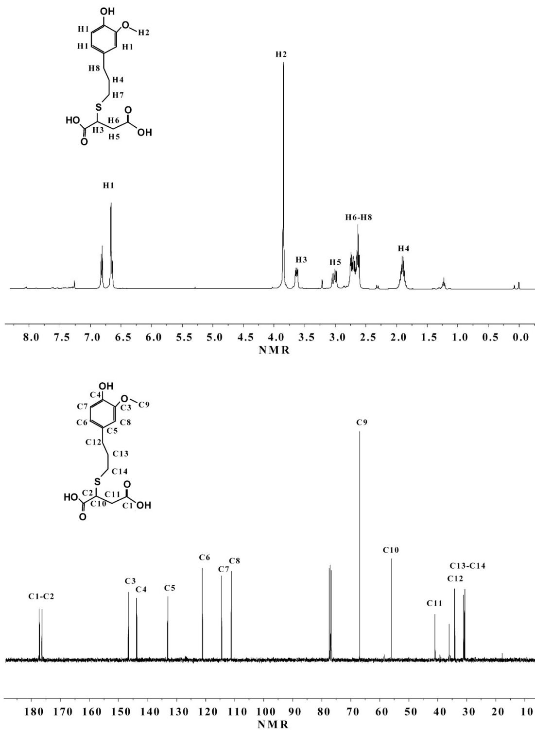
Fig. 3 The ^1\text{H} NMR and ^{13}\text{C} NMR spectra of EM3.
