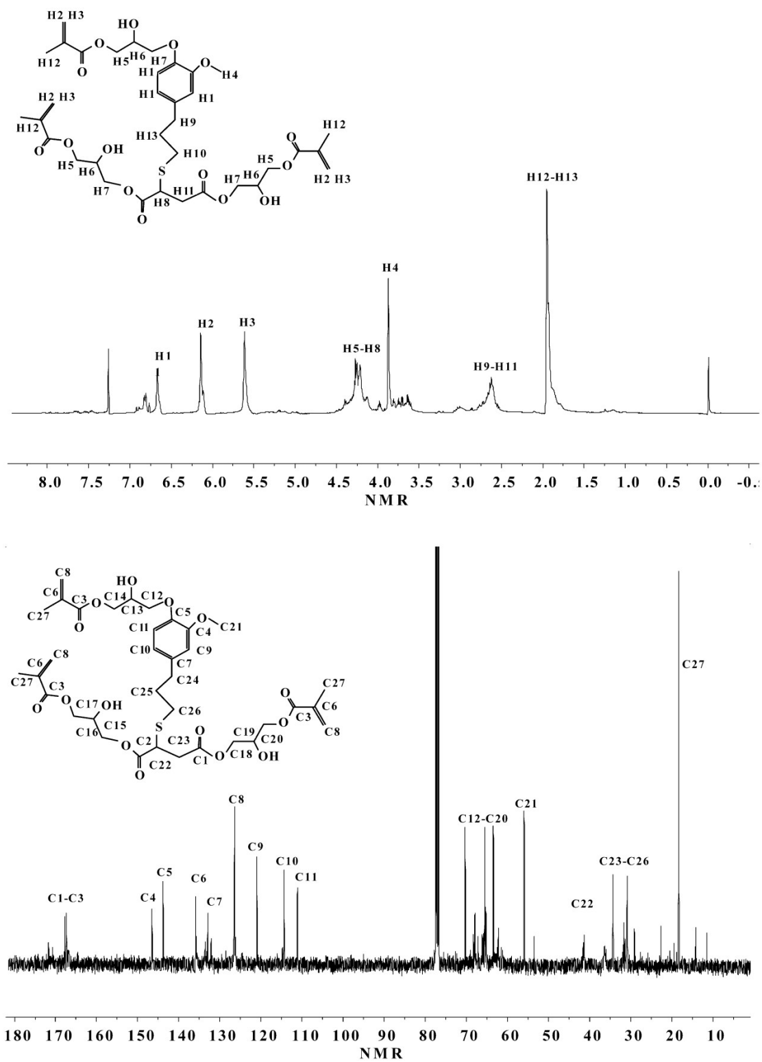
Fig. 5 The ^1\text{H} NMR and ^{13}\text{C} NMR spectra of EM3G.
