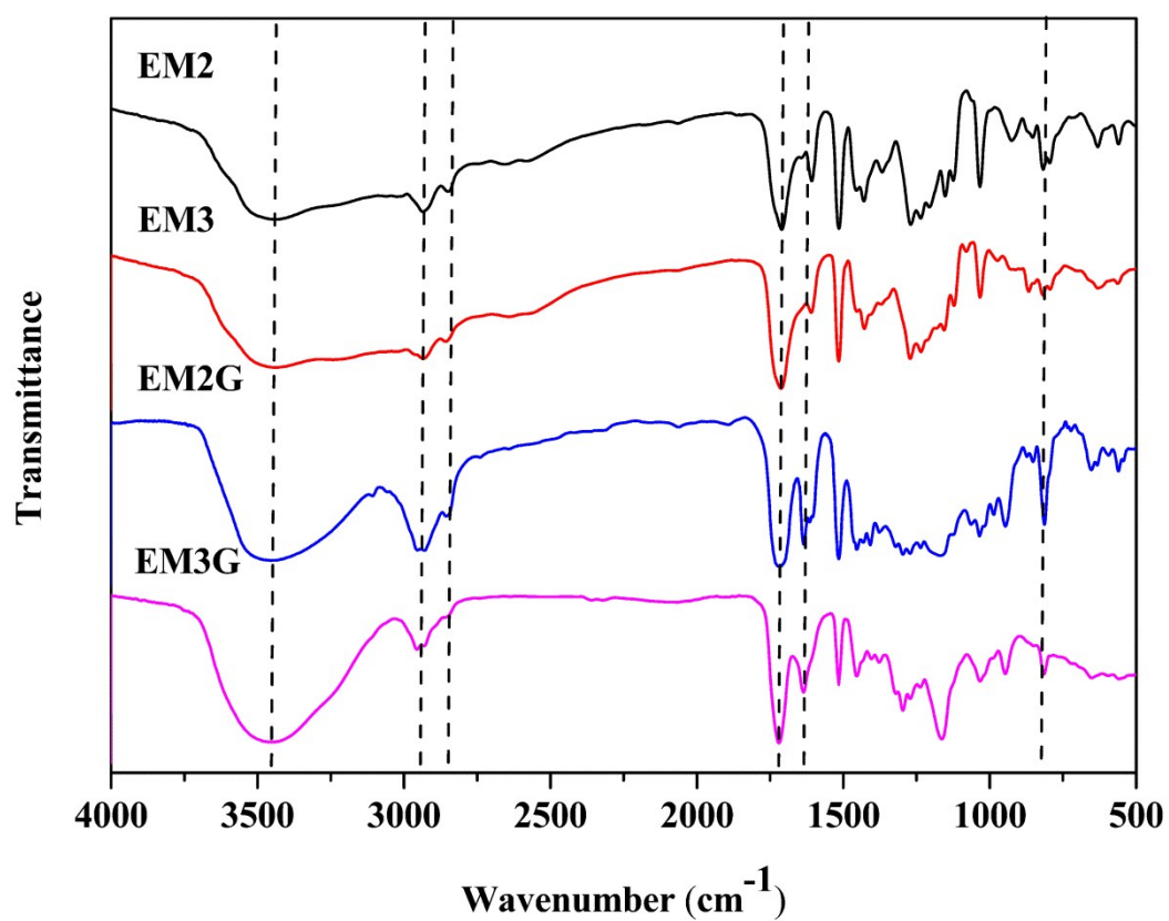
Fig. 1 FT-IR spectra of EM2, EM3, EM2G and EM3G
