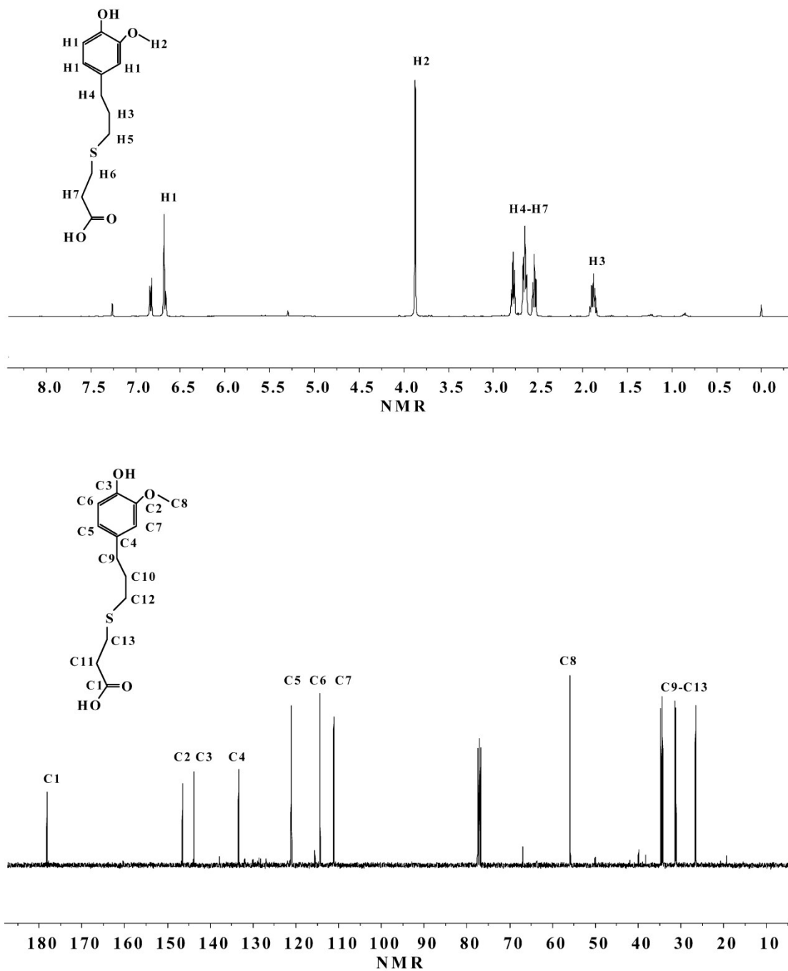
Fig. 2 The ^1\text{H} NMR and ^{13}\text{C} NMR spectra of EM2.
