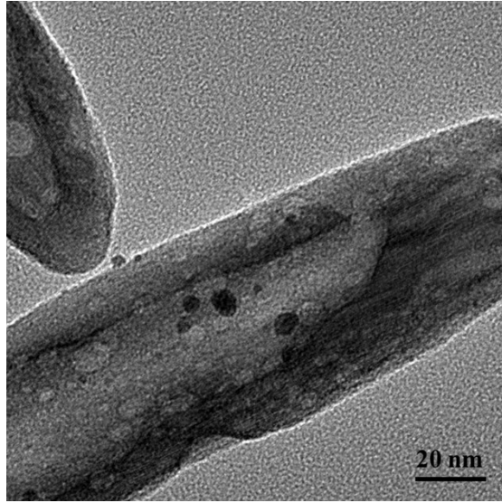
Figure S4. TEM image of Pt/Fe 2 O 3 sample after treatment in 10% H 2 O/air at 400 °C.
