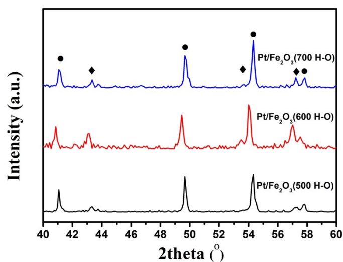
Figure S2. XRD patterns of Pt/Fe 2 O 3 after H-O treatment at different temperatures.
