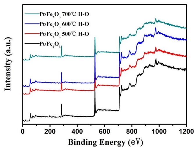
Figure S3. Survey scans of XPS spectra for Pt/Fe 2 O 3 samples before and after H-O treatment.
