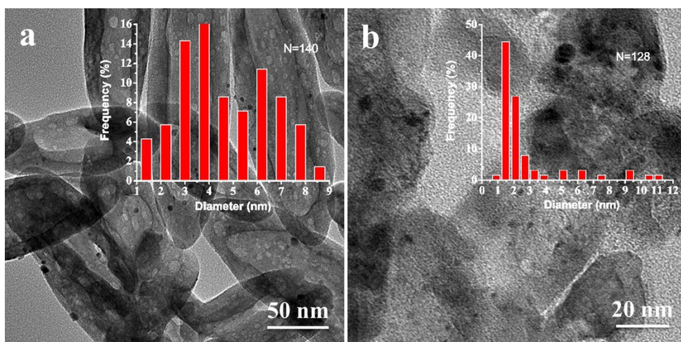
Figure S1. TEM images of Pt/Fe 2 O 3 (IM) samples before (a) and after (b) H-O treatment at 600 °C.
