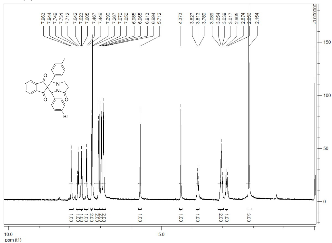
3'-(4-Bromophenyl)-1'-(p-tolyl)-6',7'-dihydro-1'H-spiro[indene-2,2'-pyrazolo[1,2-a]pyrazole]-1,3,5'(3'H)-trione (1f):
