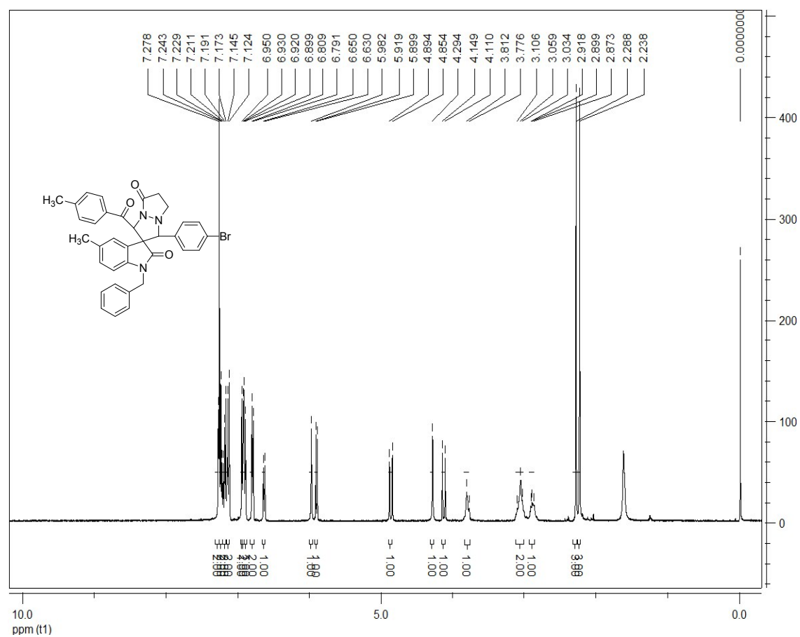
1-Benzyl-1'-(4-bromophenyl)-5-methyl-3'-(4-methylbenzoyl)-6',7'-dihydro-1'H-spiro[indoline-3,2'-pyrazolo[1,2-a]pyrazole]-2,5'(3'H)-dione (2g):
