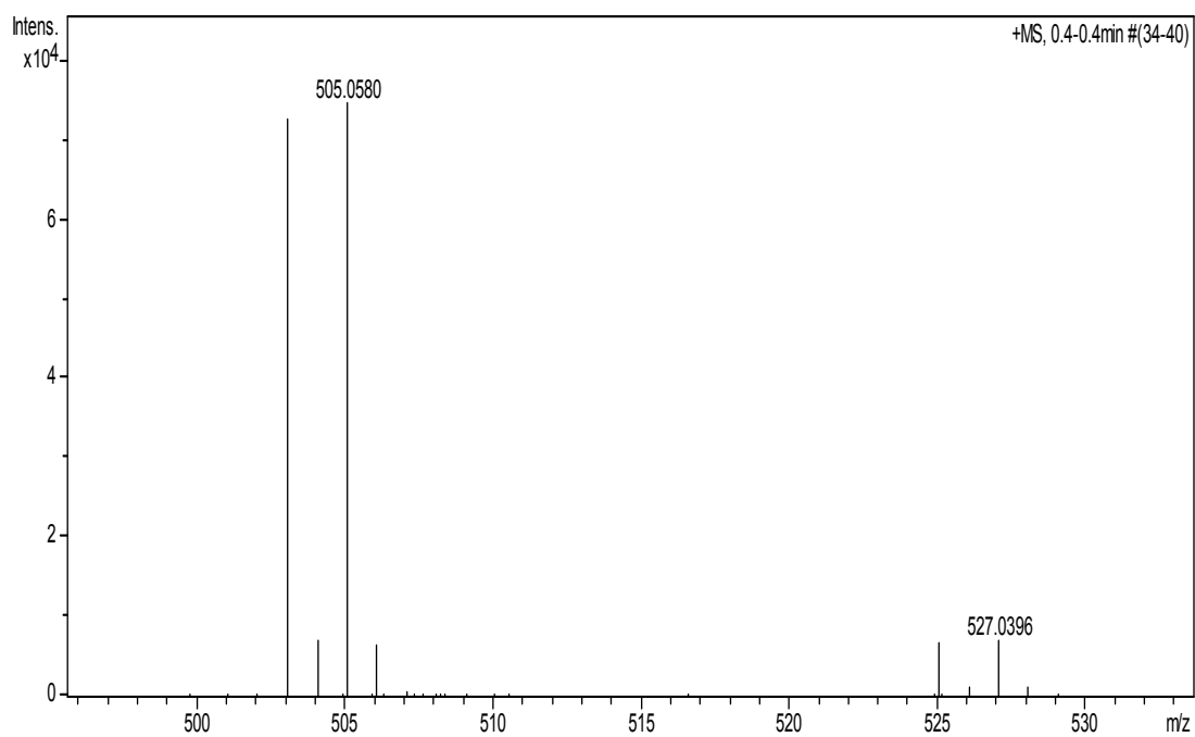
1-Benzyl-5-methyl-3'-(4-methylbenzoyl)-1'-phenyl-6',7'-dihydro-1'H-spiro[indoline-3,2'-pyrazolo[1,2-a]pyrazole]-2,5'(3'H)-dione (2a):
