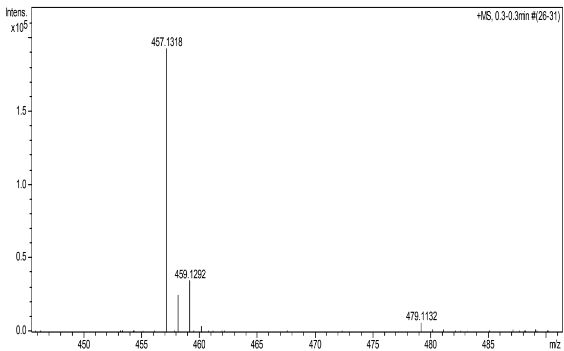
3'-(4-Bromophenyl)-1'-(p-tolyl)-6',7'-dihydro-1'H-spiro[indene-2,2'-pyrazolo[1,2-a]pyrazole]-1,3,5'(3'H)-trione (1f):
