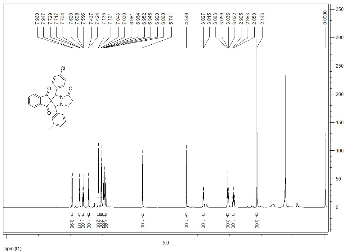
3'-(4-chlorophenyl)-1'-(m-tolyl)-6',7'-dihydro-1'H-spiro[indene-2,2'-pyrazolo[1,2-a]pyrazole]-1,3,5'(3'H)-trione (1h):
