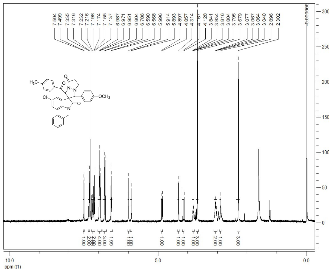
1-Benzyl-5-chloro-1'-(4-methoxyphenyl)-3'-(4-methylbenzoyl)-6',7'-dihydro-1'H-spiro[indoline-3,2'-pyrazolo[1,2-a]pyrazole]-2,5'(3'H)-dione (2e):
