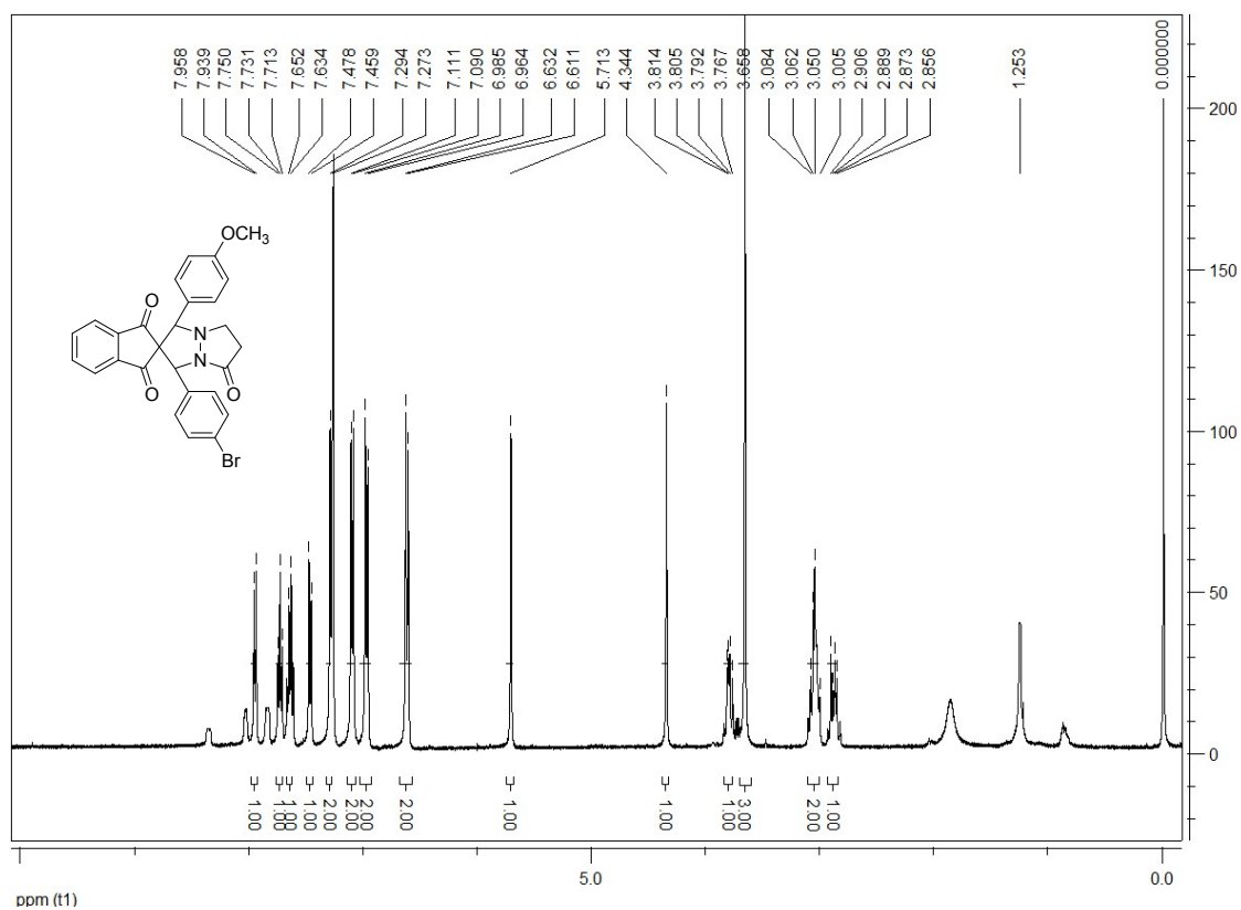
3'-(4-Bromophenyl)-1'-(4-methoxyphenyl)-6',7'-dihydro-1'H-spiro[indene-2,2'-pyrazolo[1,2-a]pyrazole]-1,3,5'(3'H)-trione (1j):
