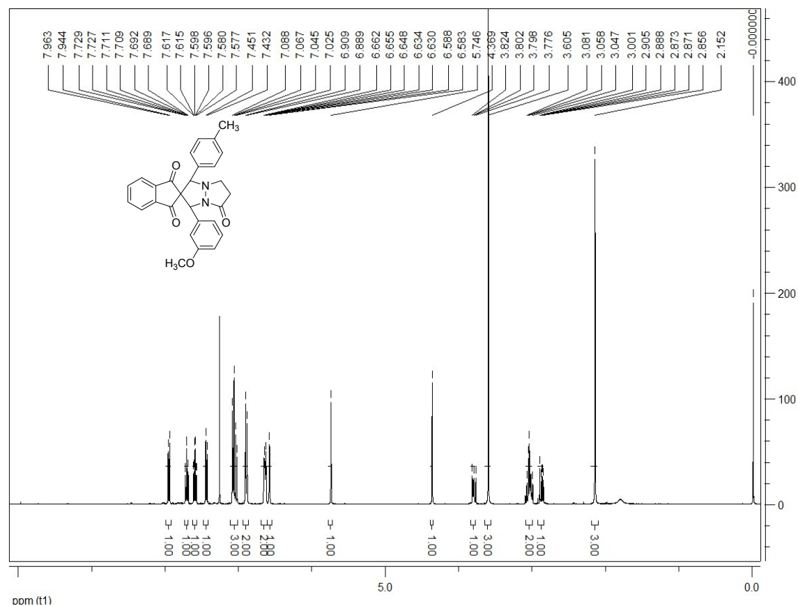
3'-(3-Methoxyphenyl)-1'-(p-tolyl)-6',7'-dihydro-1'H-spiro[indene-2,2'-pyrazolo[1,2-a]pyrazole]-1,3,5'(3'H)-trione (1d):
