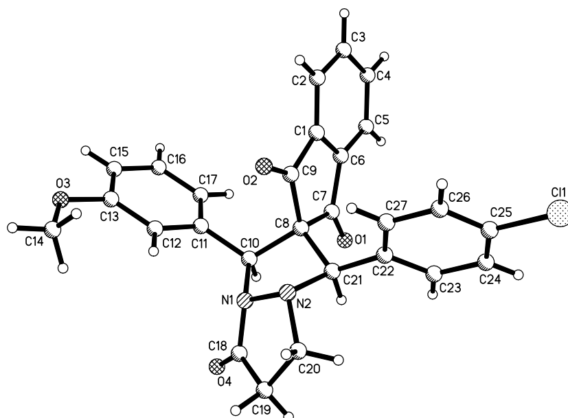
Fig. s2 Molecular structure of compound 1k
