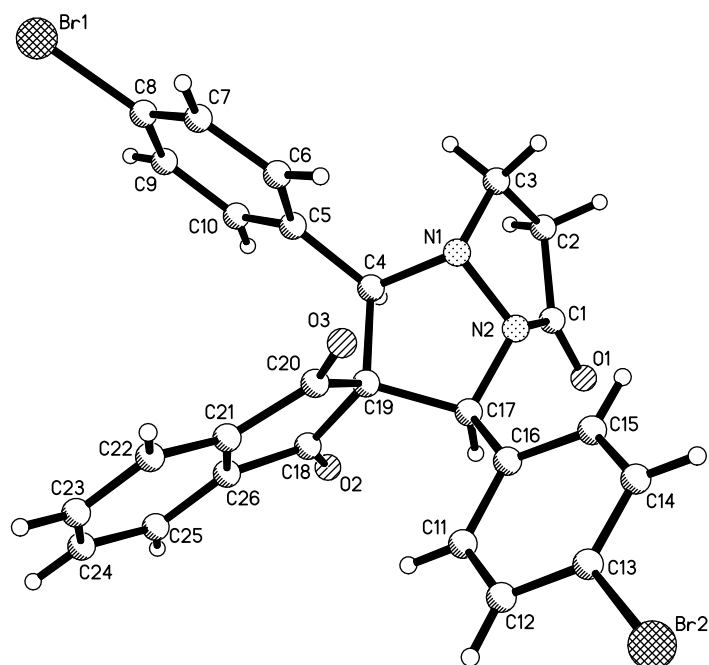
Fig. s4 Molecular structure of compound 1o
