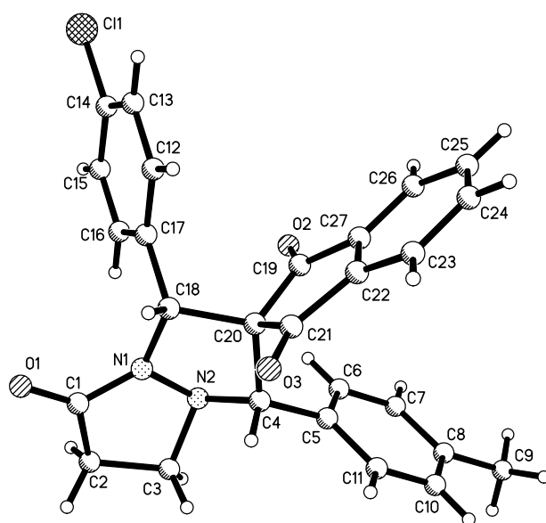
Fig s1. Molecular structure of compound 1e
