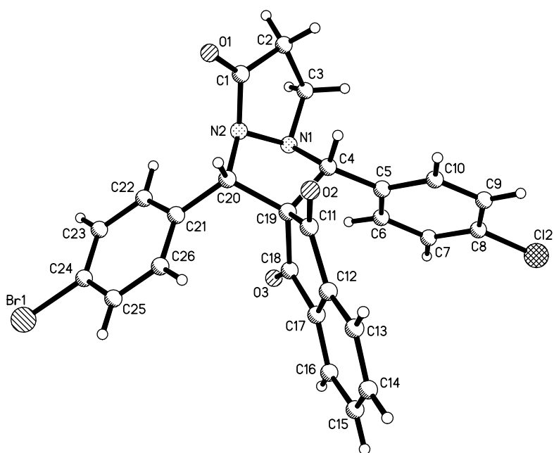
Fig. s3 Molecular structure of compound 1m
