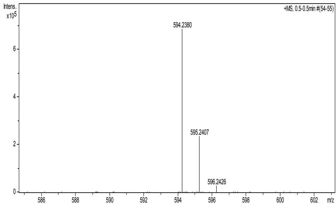
1-Benzyl-5-chloro-1'-(4-methoxyphenyl)-3'-(4-methylbenzoyl)-6',7'-dihydro-1'H-spiro[indoline-3,2'-pyrazolo[1,2-a]pyrazole]-2,5'(3'H)-dione (2e):
