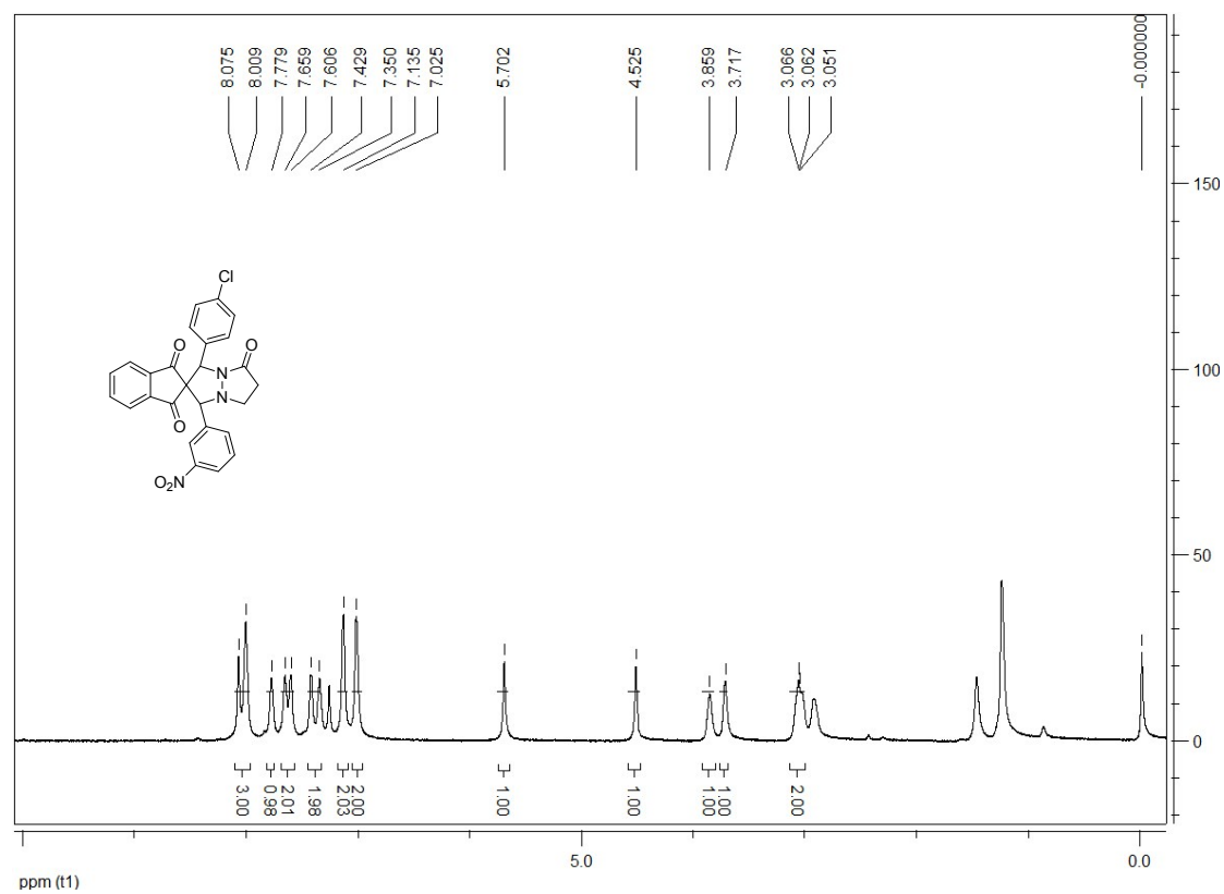
3'-(4-chlorophenyl)-1'-(3-nitrophenyl)-6',7'-dihydro-1'H-spiro[indene-2,2'-pyrazolo[1,2-a]pyrazole]-1,3,5'(3'H)-trione (1p):
