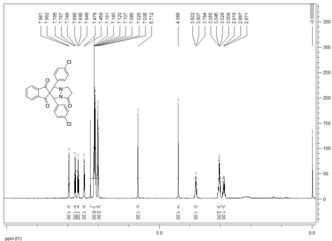
1',3'-Bis(4-chlorophenyl)-6',7'-dihydro-1'H-spiro[indene-2,2'-pyrazolo[1,2-a]pyrazole]-1,3,5'(3'H)-trione (11):
