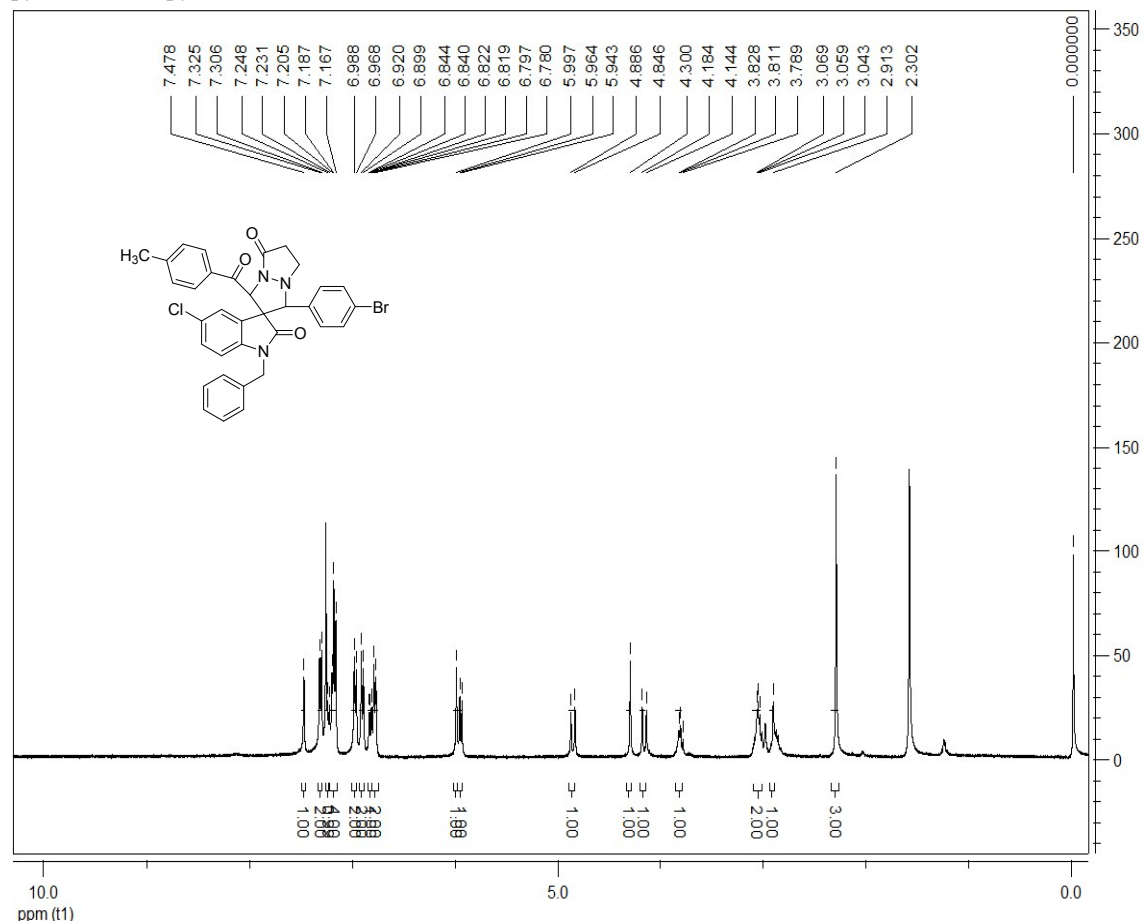
1-Benzyl-1'-(4-bromophenyl)-5-chloro-3'-(4-methylbenzoyl)-6',7'-dihydro-1'H-spiro[indoline-3,2'-pyrazolo[1,2-a]pyrazole]-2,5'(3'H)-dione (2i):
