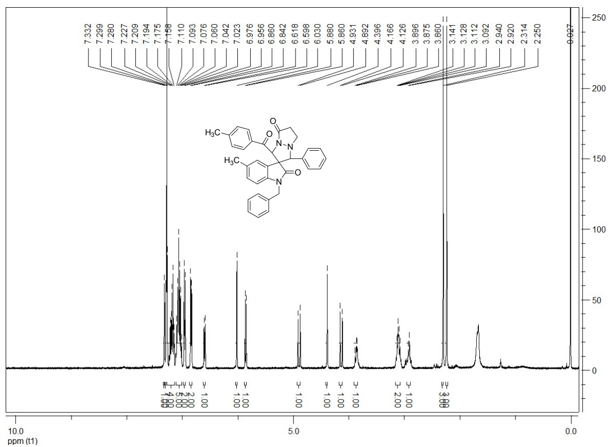
1-Benzyl-5-methyl-3'-(4-methylbenzoyl)-1'-phenyl-6',7'-dihydro-1'H-spiro[indoline-3,2'-pyrazolo[1,2-a]pyrazole]-2,5'(3'H)-dione (2a):
