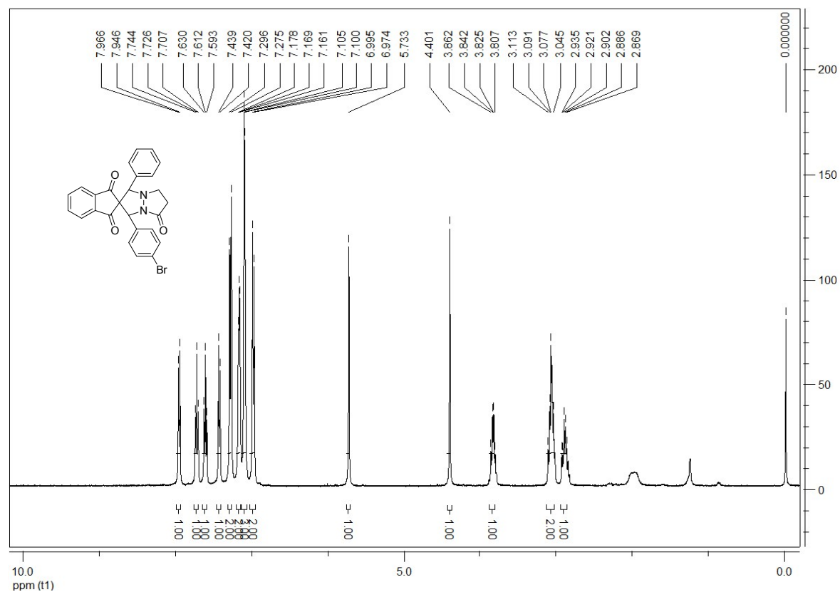
3'-(4-Bromophenyl)-1'-phenyl-6',7'-dihydro-1'H-spiro[indene-2,2'-pyrazolo[1,2-a]pyrazole]-1,3,5'(3'H)-trione (1b):
