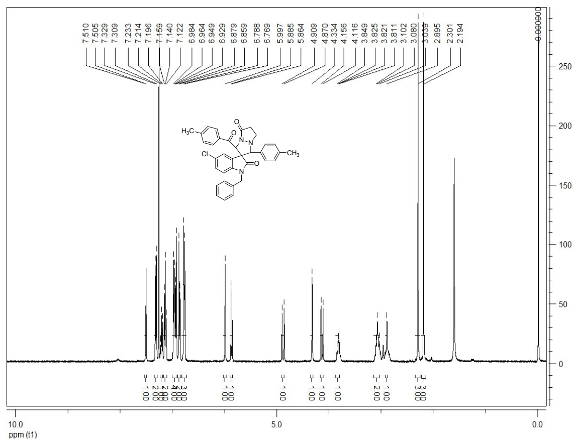
1-Benzyl-5-chloro-3'-(4-methylbenzoyl)-1'-(p-tolyl)-6',7'-dihydro-1'H-spiro[indoline-3,2'-pyrazolo[1,2-a]pyrazole]-2,5'(3'H)-dione (2c):
