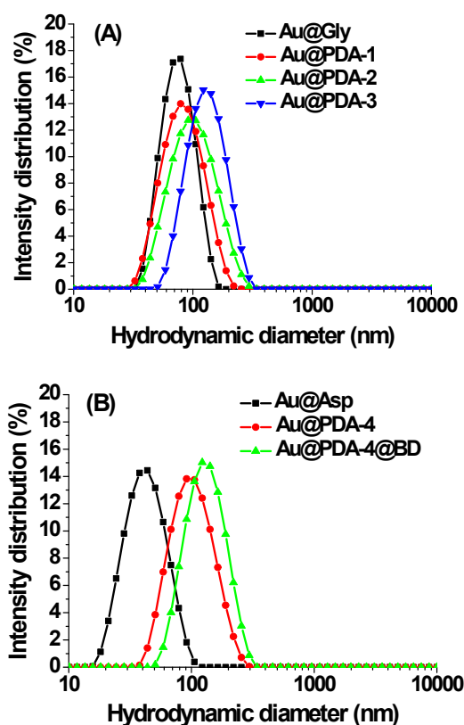
Fig. S1. Size distributions of various nanoparticles measured by dynamic light scattering.
