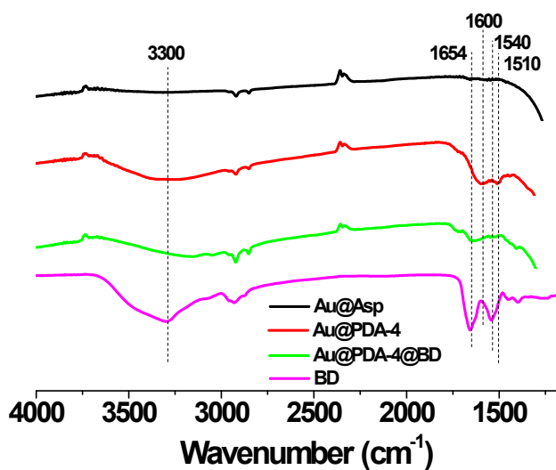
Fig. S2. FTIR spectra of Au@Asp, Au@PDA-4 and Au@PDA-4@BD nanoparticles and BD conjugate.
