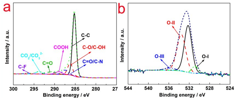
Fig. S1 C 1s (a), and O 1s (b) XPS spectra of L.
