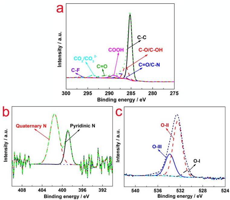
Fig. S2 C 1s (a), N 1s (b) and O 1s (c) XPS spectra of PL.
