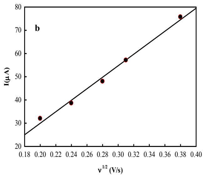
Supplementary Data 2. (a) Cyclic voltammograms (scan rate 0.04- 0.15 \text{V s}^{-1} ) for the reduction of 1 \times 10^{-4} M \text{Fe}(\text{CN})_6^{3-} in 0.1 M KCl. (b) The plot of I_{\text{pa}} versus v^{1/2} .
