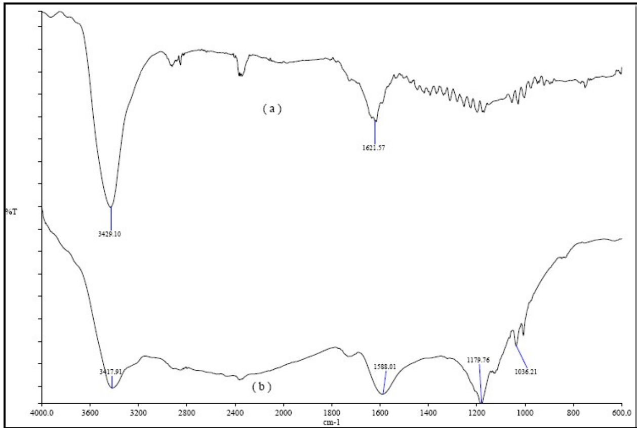
Supplementary data 1. FTIR spectra a) sulfonated-modified carbon nanoparticles b) sulfonamide-functionalized carbon nanoparticles
