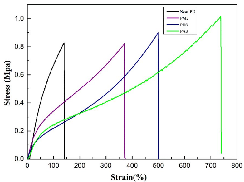
Figure S3. Stain-stress curves of neat PU, PM3, PD3, and PA3.
