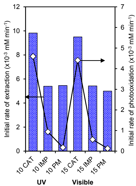
Fig. S2 Effect of different catalysts on sulfur removal under UV and visible region.
