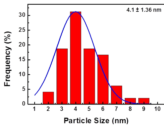
Figure S2. Particles size distribution histograms of Pd-3 catalyst after 10 cycles hydrogenation of 4-nitrotoluene.
