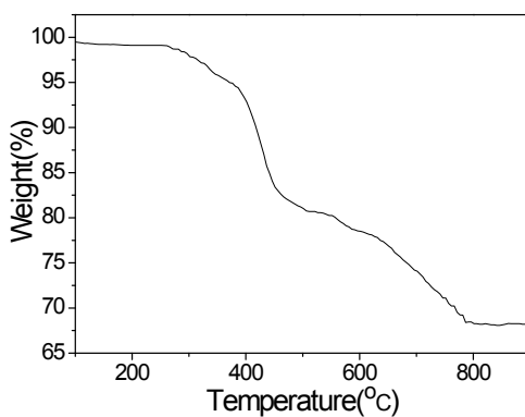
Fig 1S TG of rGO/CuI/PANI nanocomposites.
