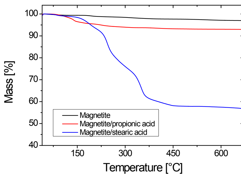
Figure S1. Thermogravimetric analysis of magnetite nanoparticles with different surface functionalizations.
