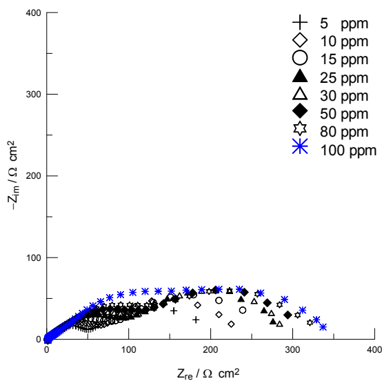
Figure S1. Nyquist diagram of phenol alkyne for API 5L X52 steel immersed in 1 M HCl under static conditions.
