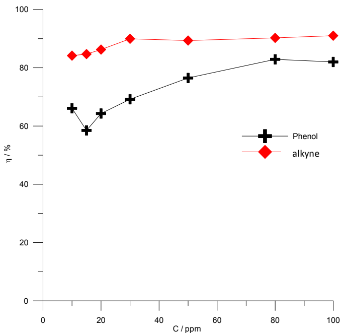
Figure S2. Inhibition efficiency variation when phenol and its corresponding alkyne were evaluated as a function of concentration for API 5L X52 steel immersed in 1 M HCl.
