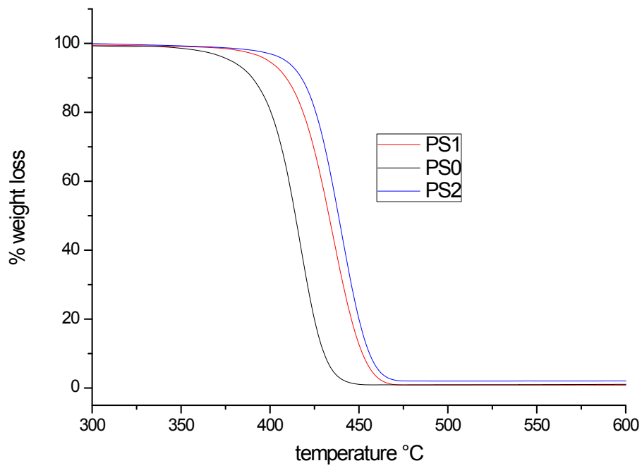
SF5: TGA curves of blank experiment (PS0) and composites with 2D BP nanolayers (samples PS1 and PS2)
