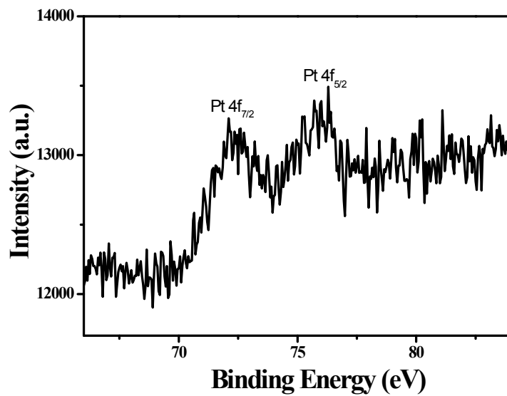
Fig. S1 The high-resolution XPS spectra of Pt 4f for Ti(IV)-Pt/Bi 2 WO 6 (5 wt%).
