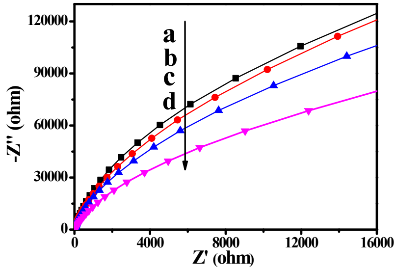
Fig. S2 Electrochemical impedance spectra for various samples: (a) \text{Bi}_2\text{WO}_6 ; (b) \text{Ti(IV)/Bi}_2\text{WO}_6 (5 wt%); (c) \text{Pt/Bi}_2\text{WO}_6 ; (d) \text{Ti(IV)-Pt/Bi}_2\text{WO}_6 (5 wt%).
