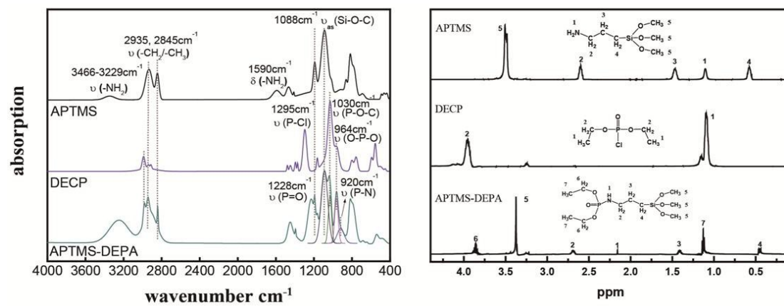
Fig. S1 IR (left) and 1 H-NMR (right) spectra of APTMS, DECP and APTMS-DEPA
