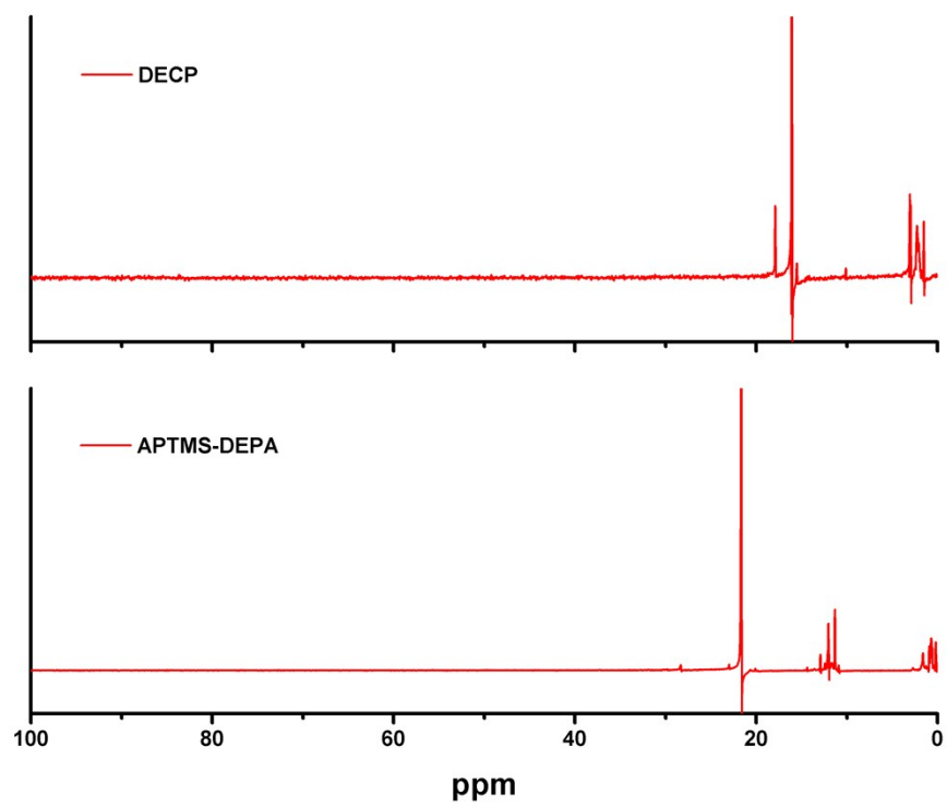
Fig. S2 ^{31}\text{P} NMR spectra for DECP and APTMS-DEPA
