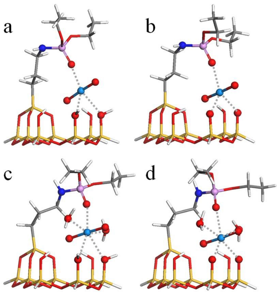
Fig. S4 Full optimized structures for four possible situations
