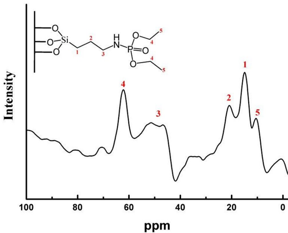
Fig. S3 ^{13}\text{C} NMR spectrum for SBA-12.5%DEPA
