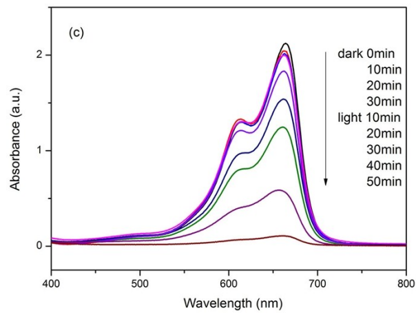
Figure S2 The changes of time-dependent UV-Vis absorbance spectra in the presence of (a)G3, (b)U3 and (c)UC3 for different times.
