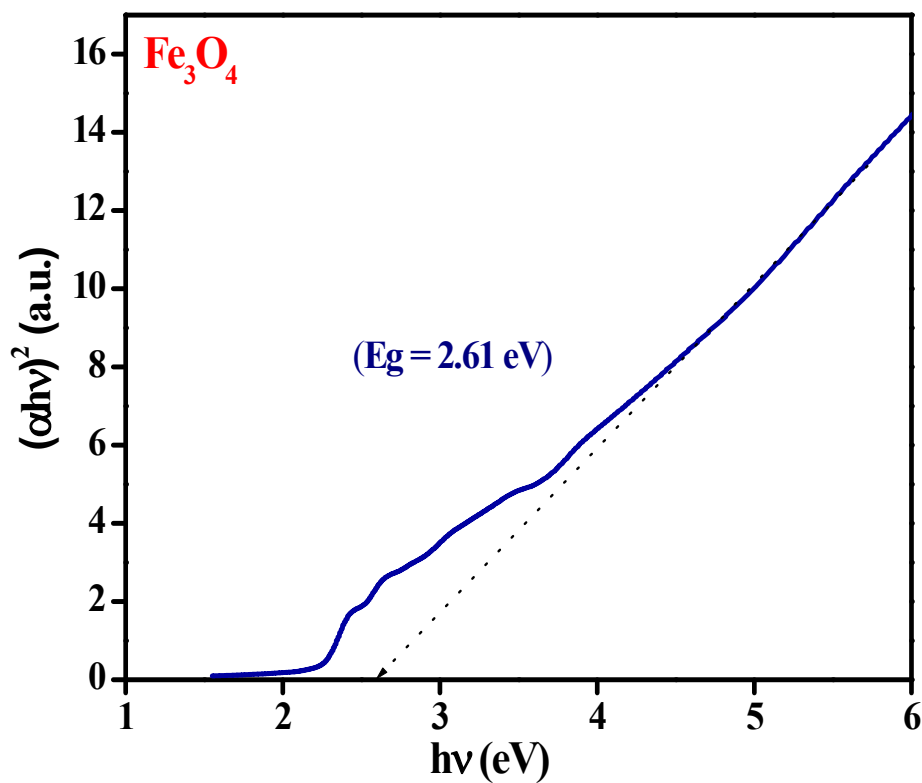
Fig. S1. Band gap plot of pure \text{Fe}_3\text{O}_4 .
