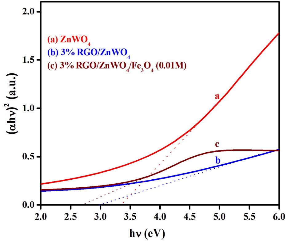
Fig. S2. Band gap plots for (a) ZnWO_4 , (b) RGO/ ZnWO_4 and (c) RGO/ ZnWO_4/Fe_3O_4 .
