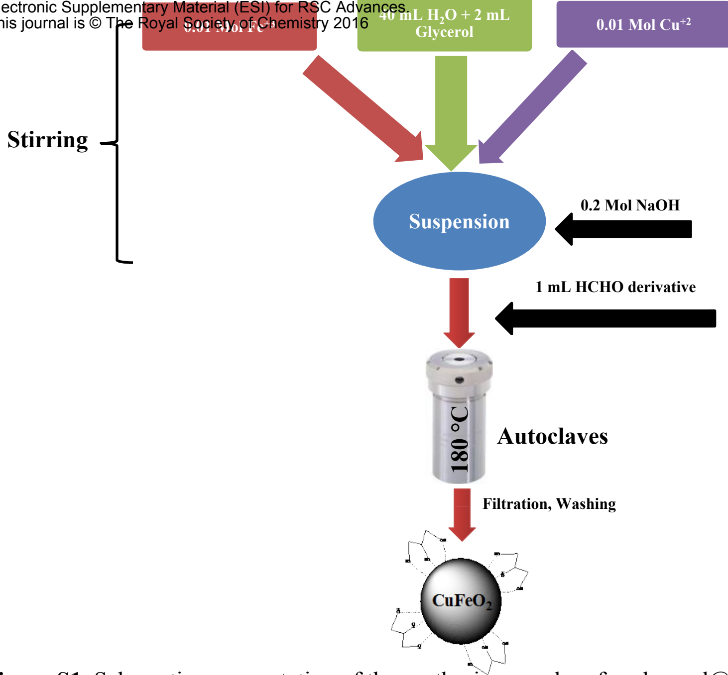
Figure S1. Schematic representation of the synthesis procedure for glycerol@CuFeO 2 NPs
