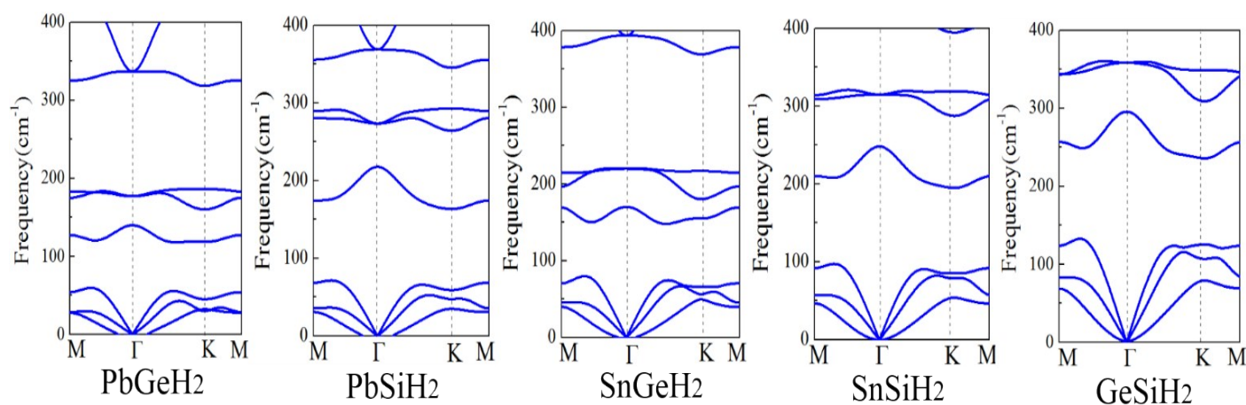
Fig. S1 The calculated phonon band spectrum for PbGeH 2 , PbSiH 2 , SnGeH 2 , SnSiH 2 , GeSiH 2 films, respectively.
