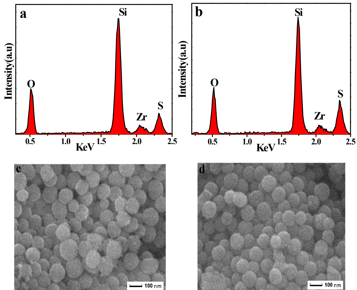
Fig. S2. EDS and SEM images of non-SZs (a, c) and meso-SZs (b, d).
