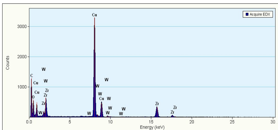
Figure. S1 EDX patterns of as-prepared mesoporous nano- \text{WO}_x/\text{ZrO}_2 catalyst. The as-prepared product have rich Zr and W components.
