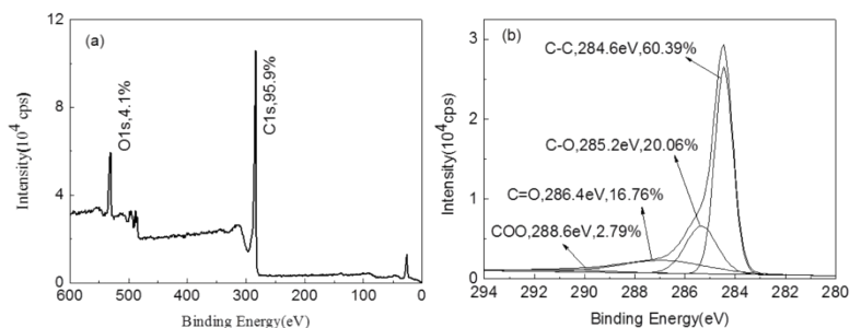
Figure.S1. XPS curves of pristine MWCNTs, (a) wide scan, (b) C1s narrow scan
