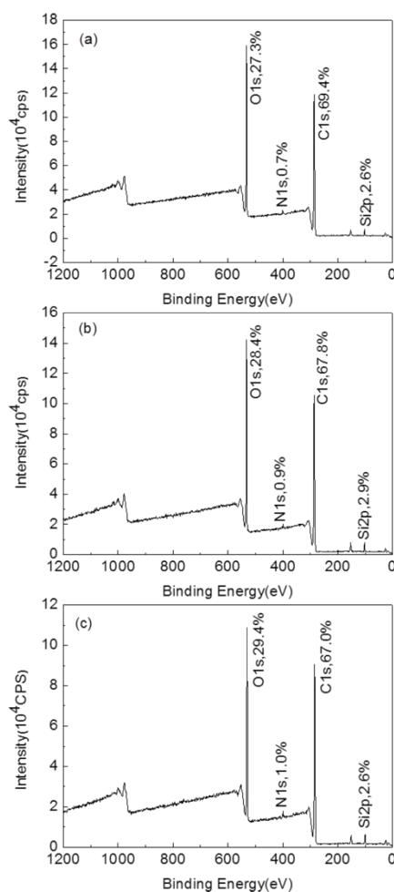
Figure.S3. XPS curves of wide scan of MWCNTs-NOHMs, (a) MWCNTs-NOHM-3h, (b) MWCNTs-NOHM-5h, (c) MWCNTs-NOHM-7h
