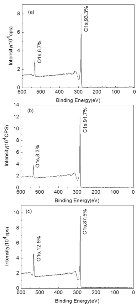
Figure.S2. XPS curves of wide scan of acid MWCNTs, (a) MWCNTs-3h, (b) MWCNTs-5h, (c) MWCNTs-7h
