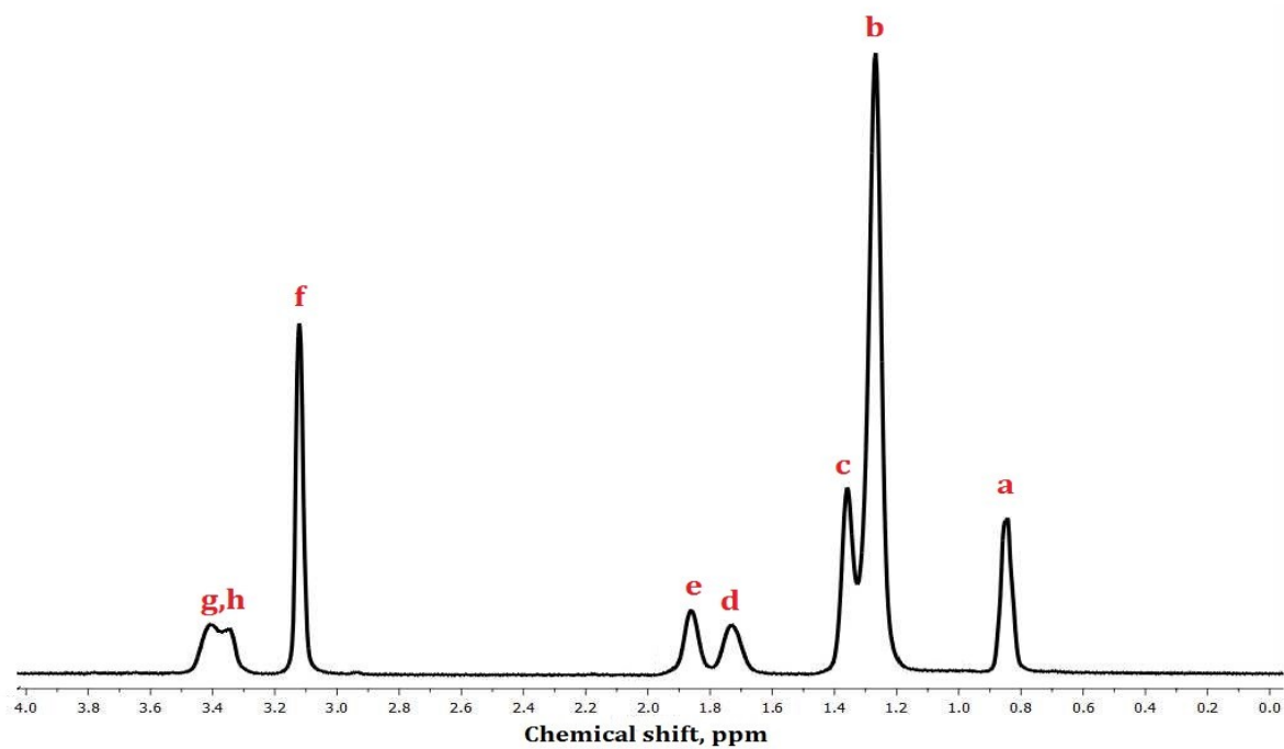
SM1: 1 H NMR spectrum of 50 mM 12-4-12 at 30 °C
