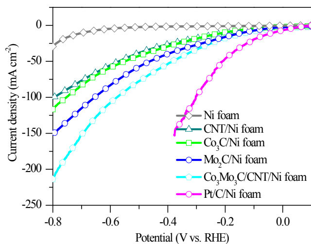
Fig. S1. Polarization curves of various electrodes.
