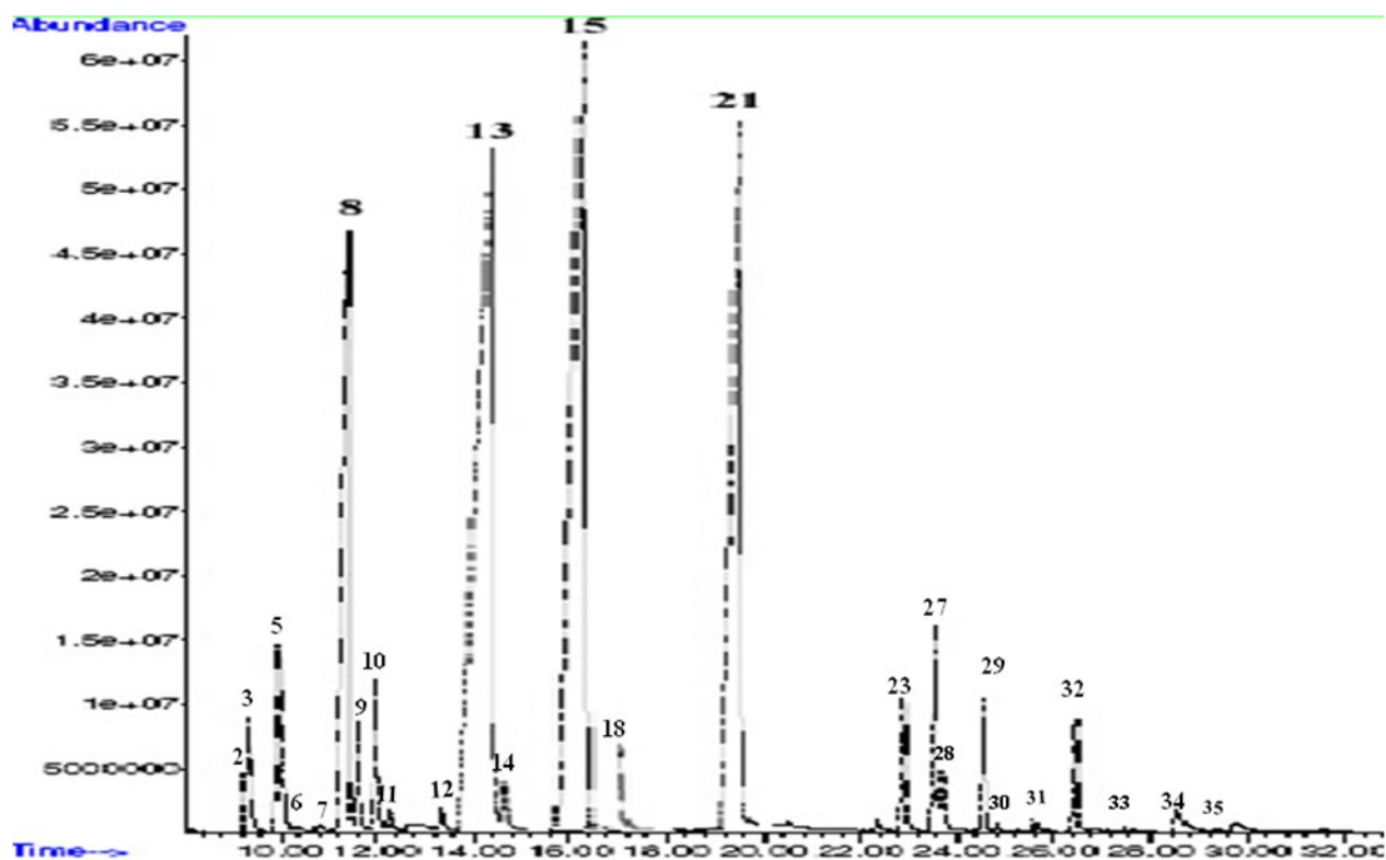
Figure 1S: Total ion chromatogram of the essential oil of A. herba-alba . Numbers referred to the main components (Table 1).
