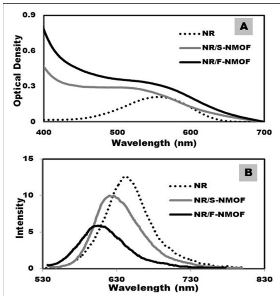
Figure S1: (A) Absorption, and (B) fluorescence emission spectra of free (NR) and nanoencapsulated (NR/S-NMOF and NR/F-NMOF) fluorophores.
