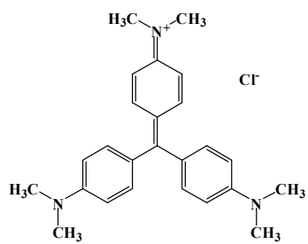
Methyl violet (MV)
