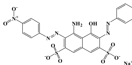
Amino black 10B (AB10B)
