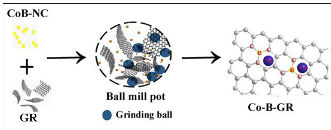
Scheme S1. Illustration of the formation process of Co-B-GR with a ball-milling method.
