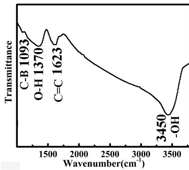
Figure S1. FT-IR spectrum of the as-obtained Co-B-GR.
