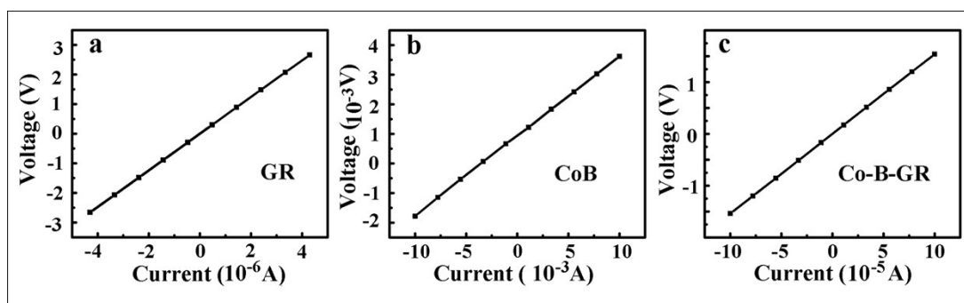
Figure S2. Electrical conductivities of amorphous GR and CoB reactants, and the Co-B-GR hybrid product.
