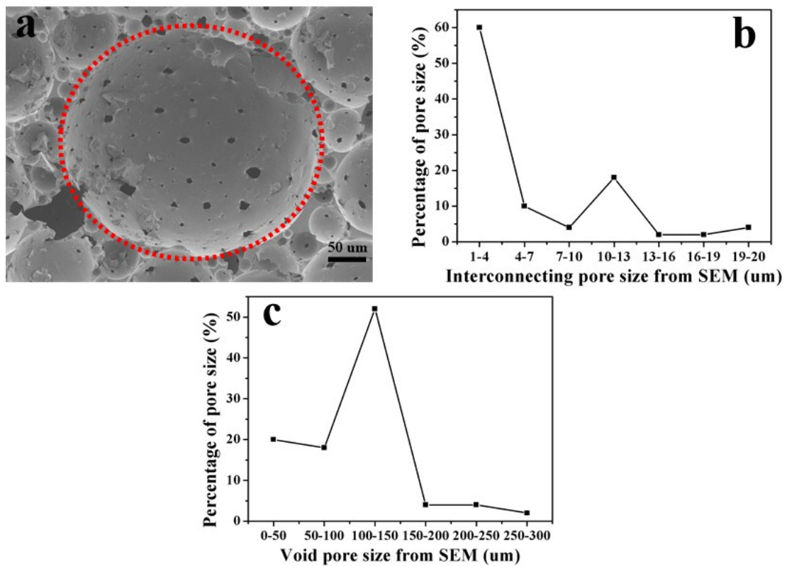
Fig. S2 Partial enlarged SEM image of UFMF11 (a), interconnecting (b) and void pore size distribution from SEM image of UFMF11 (c).
