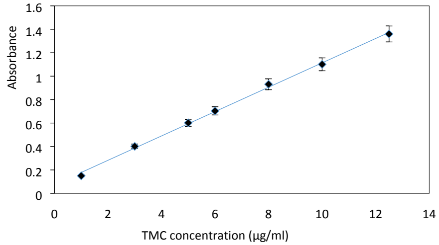
Figure S2: Standard calibration curve of tamoxifen citrate at the wavelength of \lambda=237 nm.
