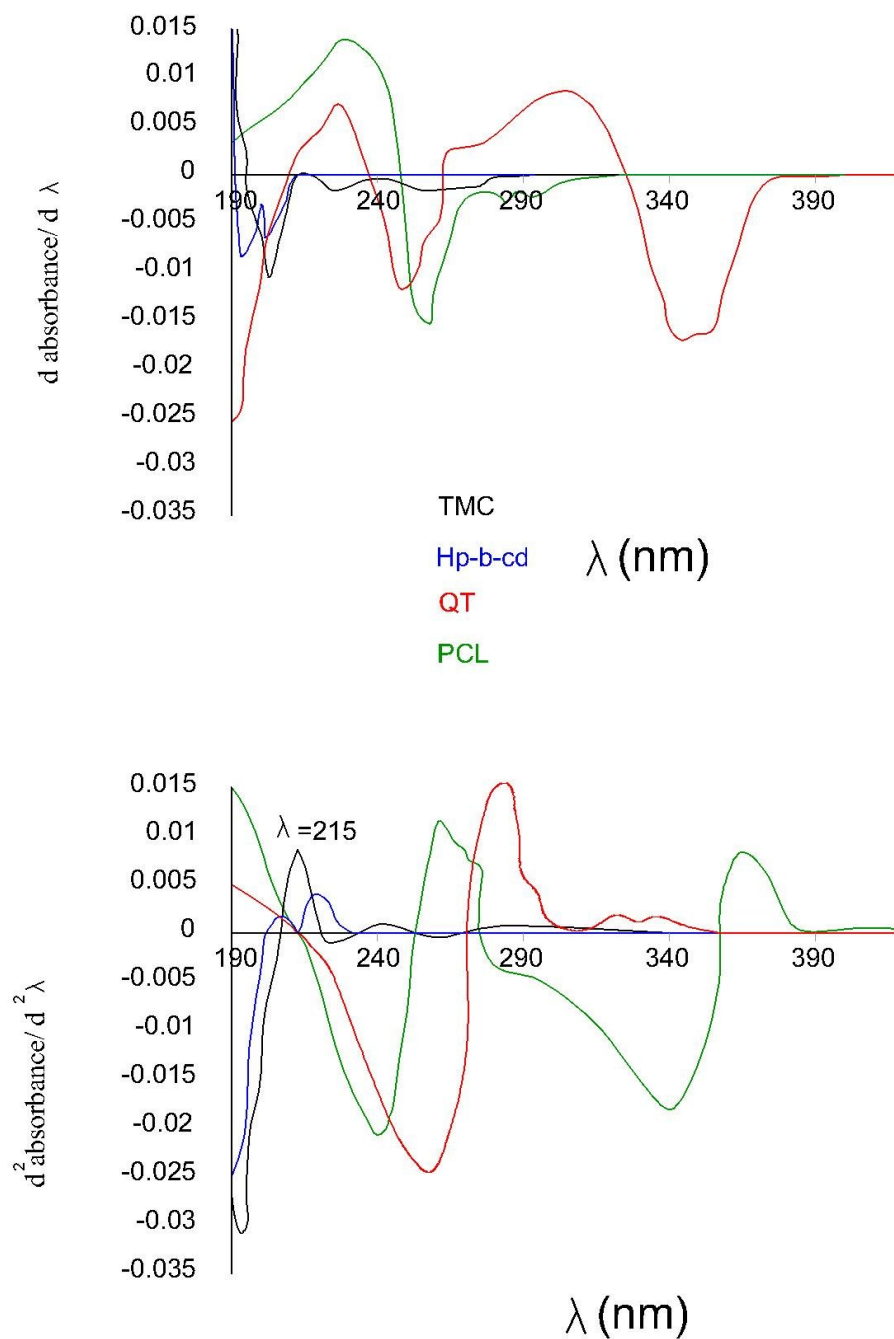
Figure S1: First (a) and second (b) derivative UV spectra of TMC, QT, PCL and 2Hp- \beta -CD
