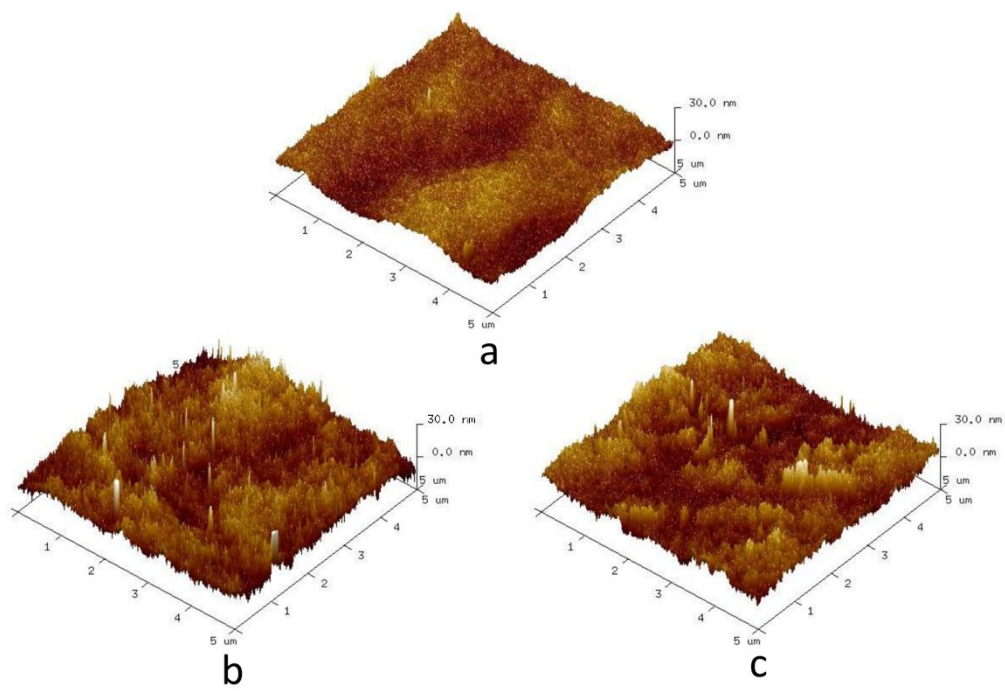
Fig. S2 AFM 3D images of membranes: (a) PES, (b) PES-L and (c) PES-H.
