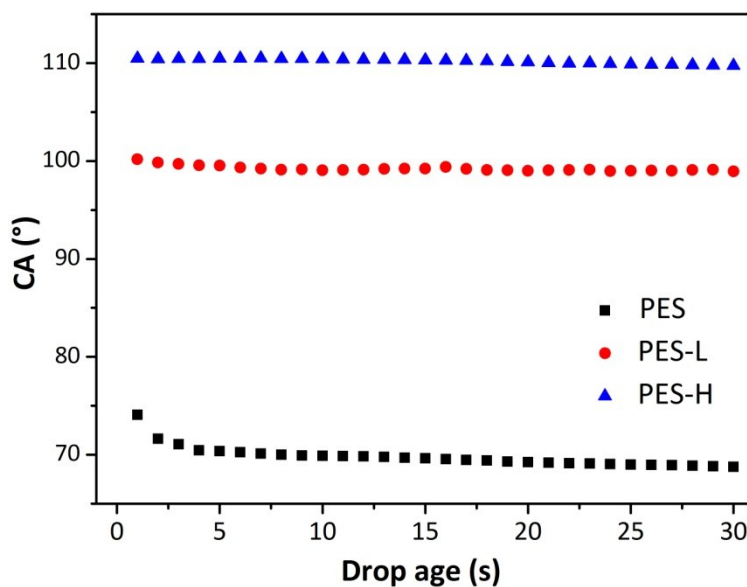
Fig. S1 Static CA evolution of PES, PES-L and PES-H membranes versus drop age.
