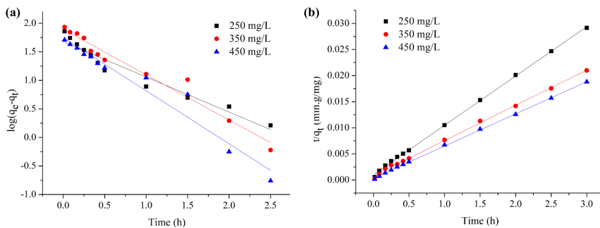
Supplemental Material 1 The fitted plots of the pseudo-first-order model (a) and pseudo-second-order kinetic model (b)
