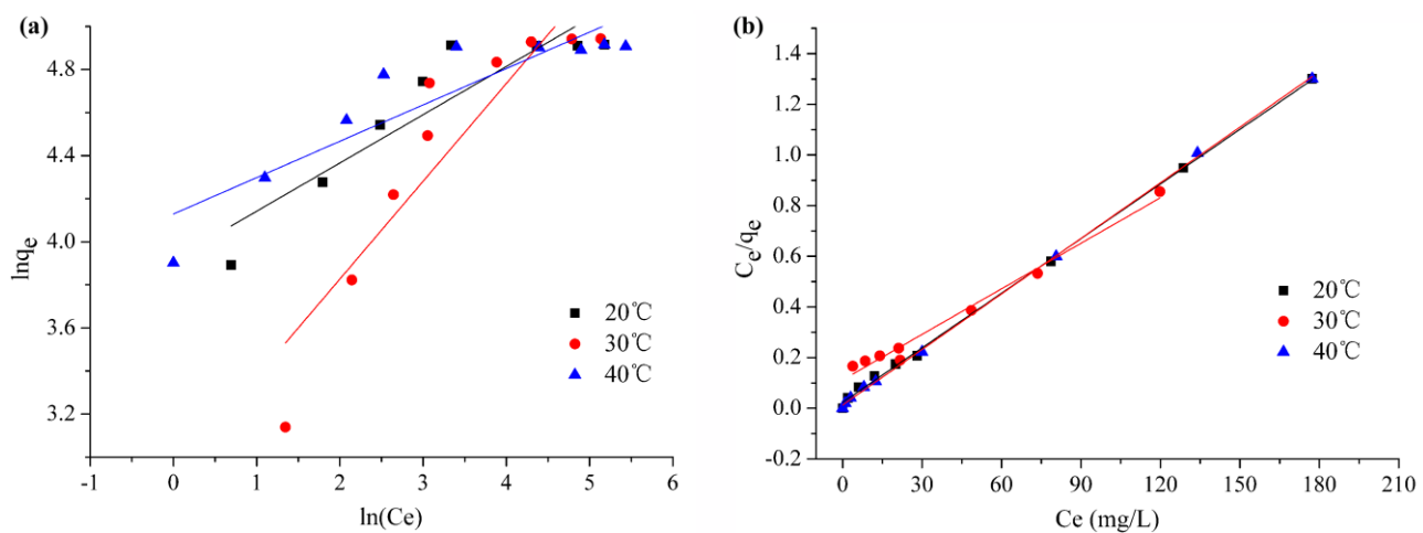
Supplemental Material 2 The fitted plots of Freundlich equation (a) and Langmuir equation (b)
