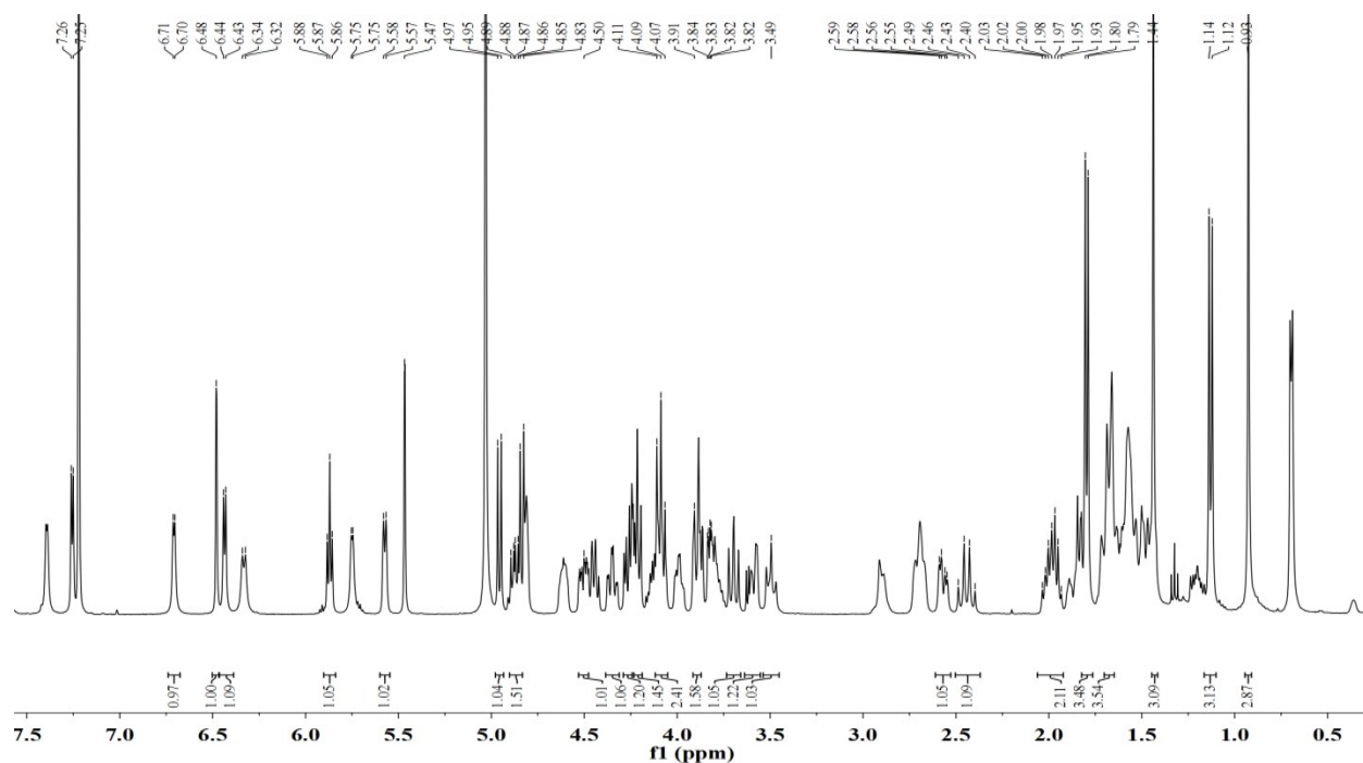
Figure S29. ^1\text{H} NMR spectrum of compound 5 (pyridine- d_5 )
