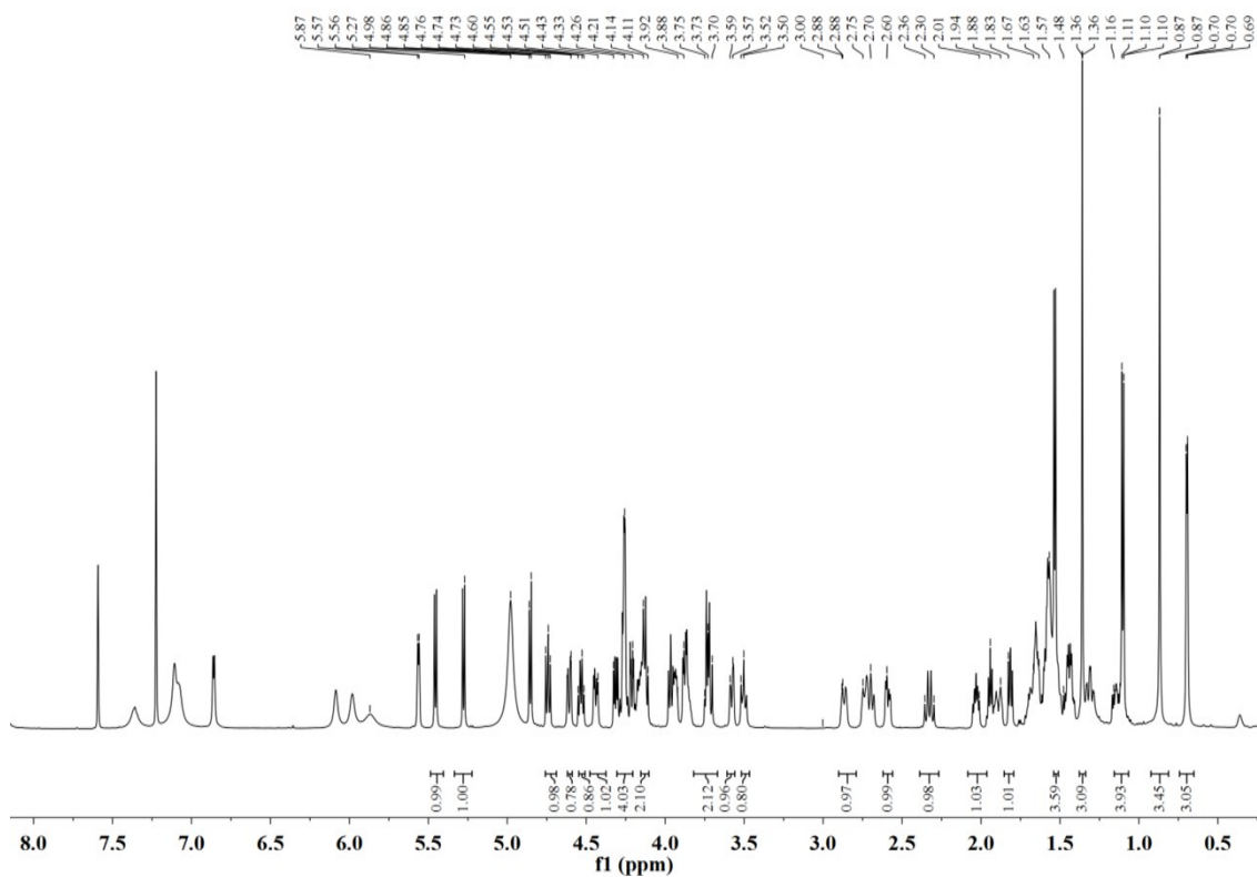
Figure 73. ^{13}\text{C} NMR spectrum of compound 12 (pyridine- d_5 )
