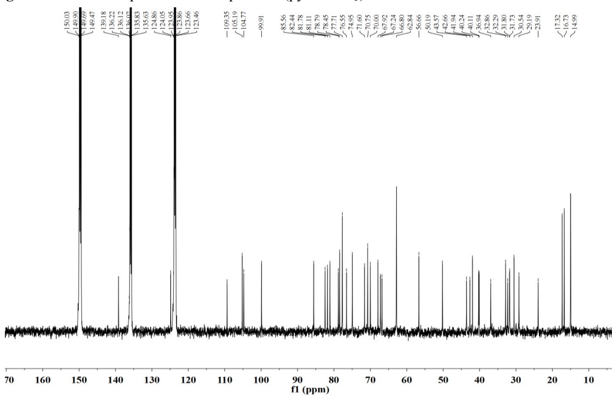
Figure S9. ^{13}\text{C} NMR spectrum of compound 2 (pyridine- d_5 )
