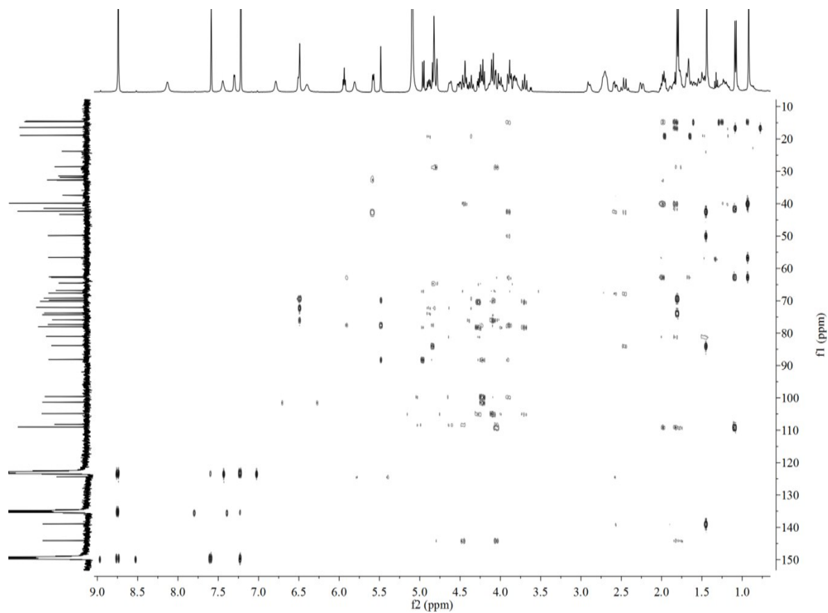
Figure S59. HMBC NMR spectrum of compound 9 (pyridine- d_5 )
