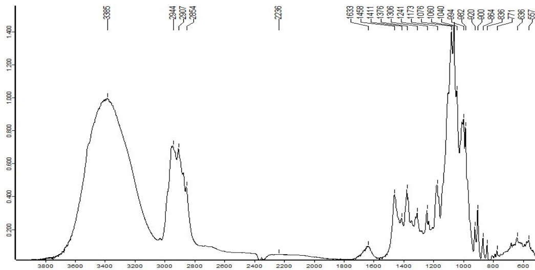
Figure S48. IR (KBr, disc) spectrum of compound 7
