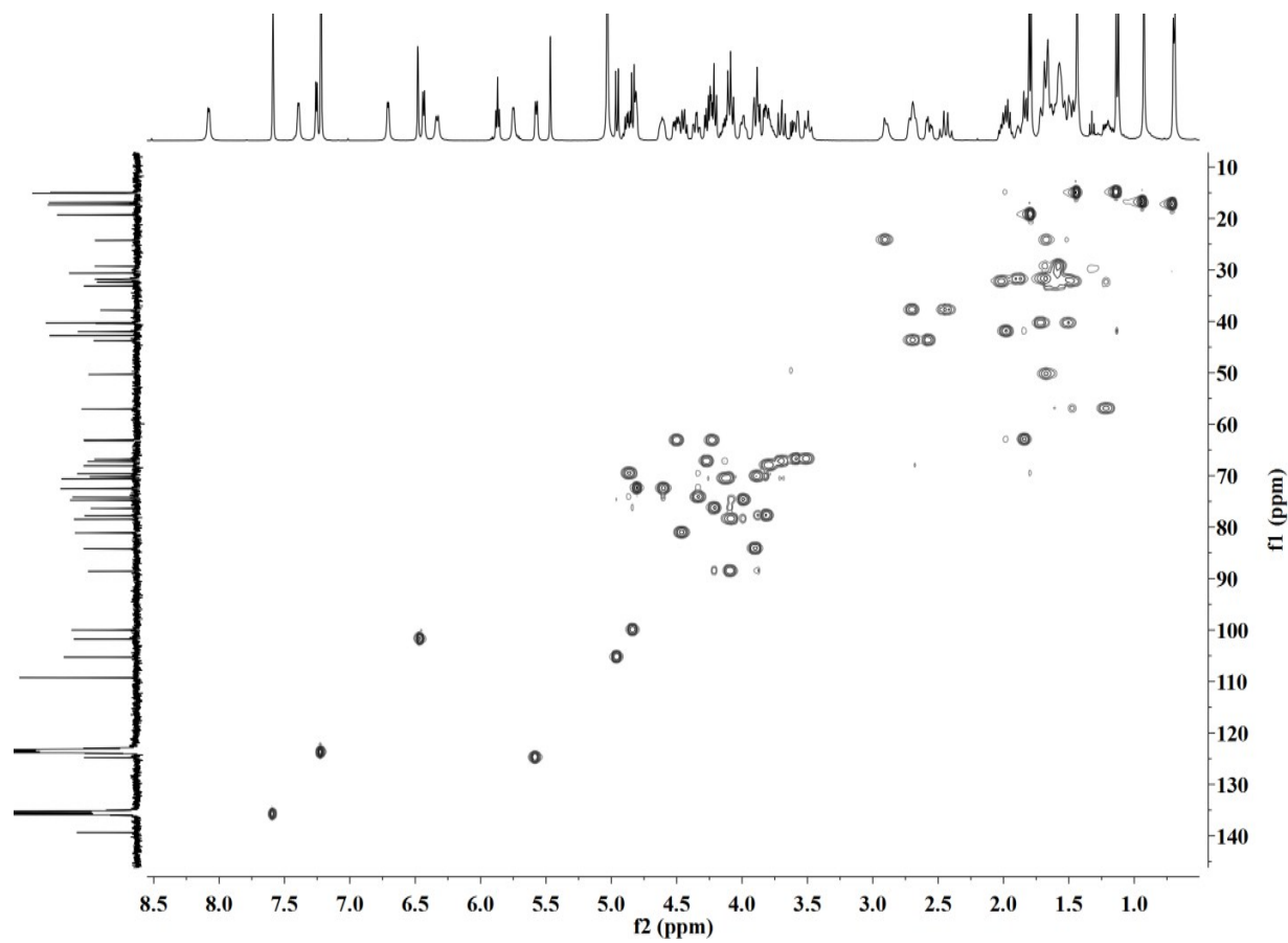
Figure S31. HSQC NMR spectrum of compound 5 (pyridine- d_5 )
