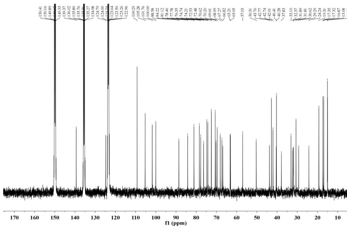
Figure S43. ^{13}\text{C} NMR spectrum of compound 7 (pyridine- d_5 )
