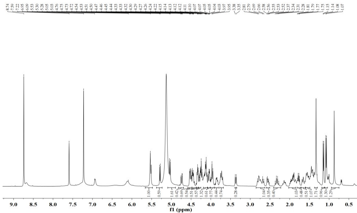
Figure S1. ^1\text{H} NMR spectrum of compound 1 (pyridine- d_5 )
