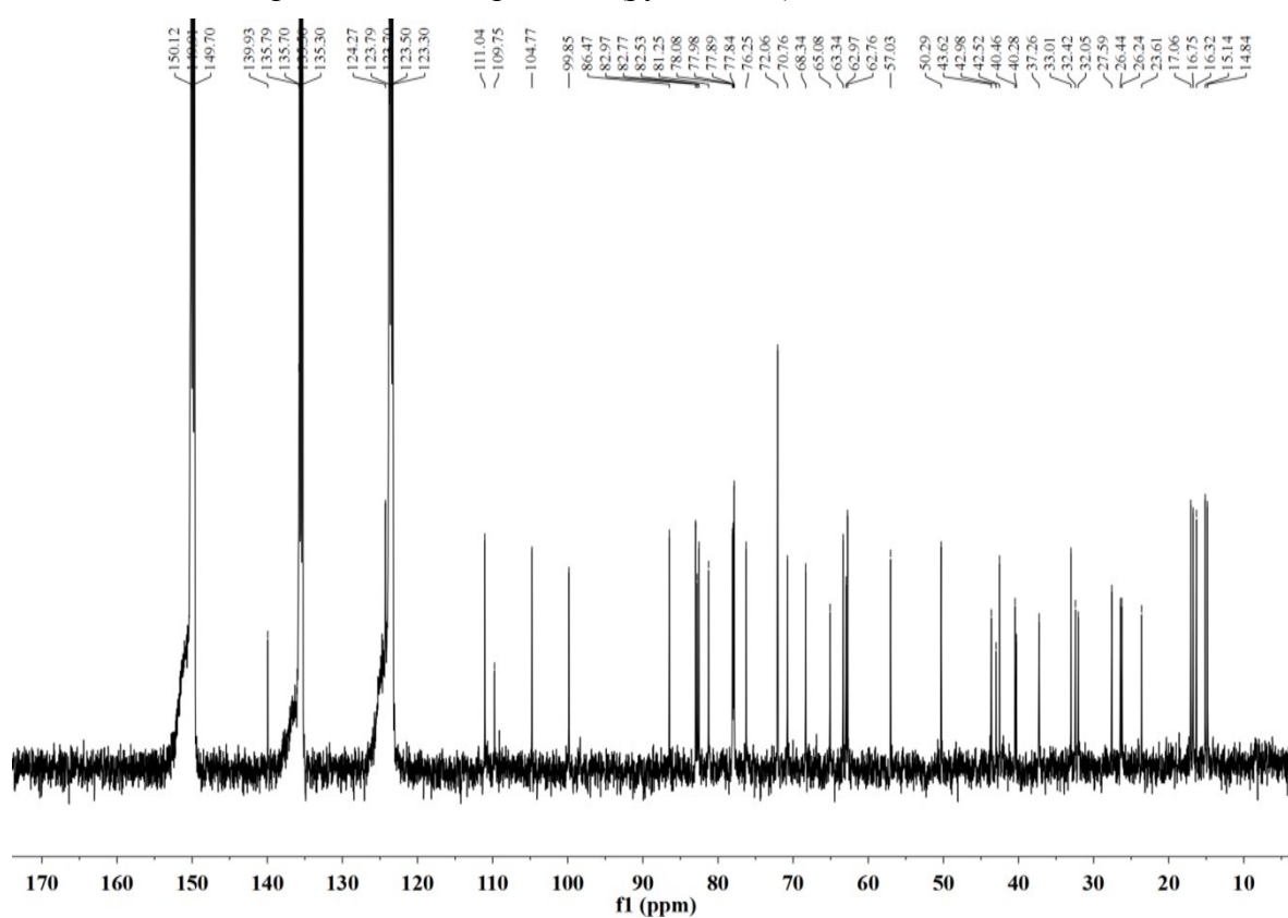
Figure S38. HSQC NMR spectrum of compound 6 (pyridine- d_5 )
