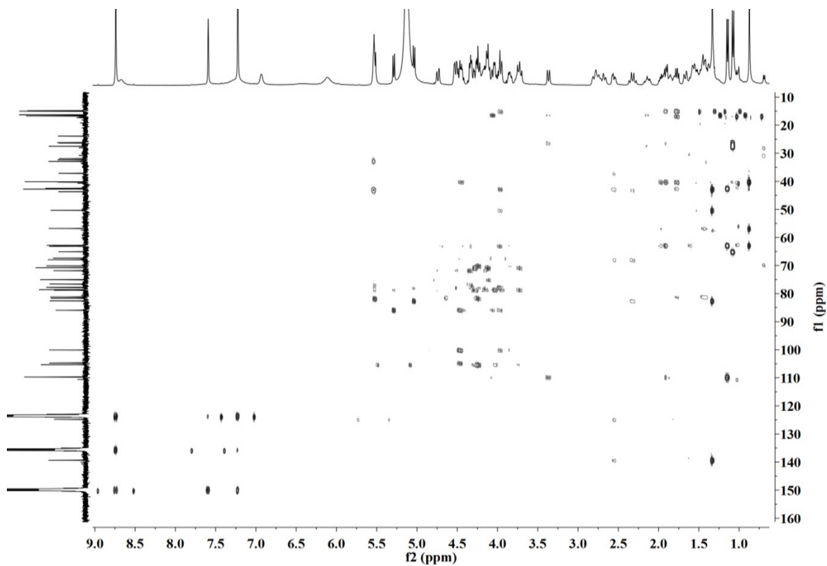
Figure S4. HMBC NMR spectrum of compound 1 (pyridine- d_5 )
