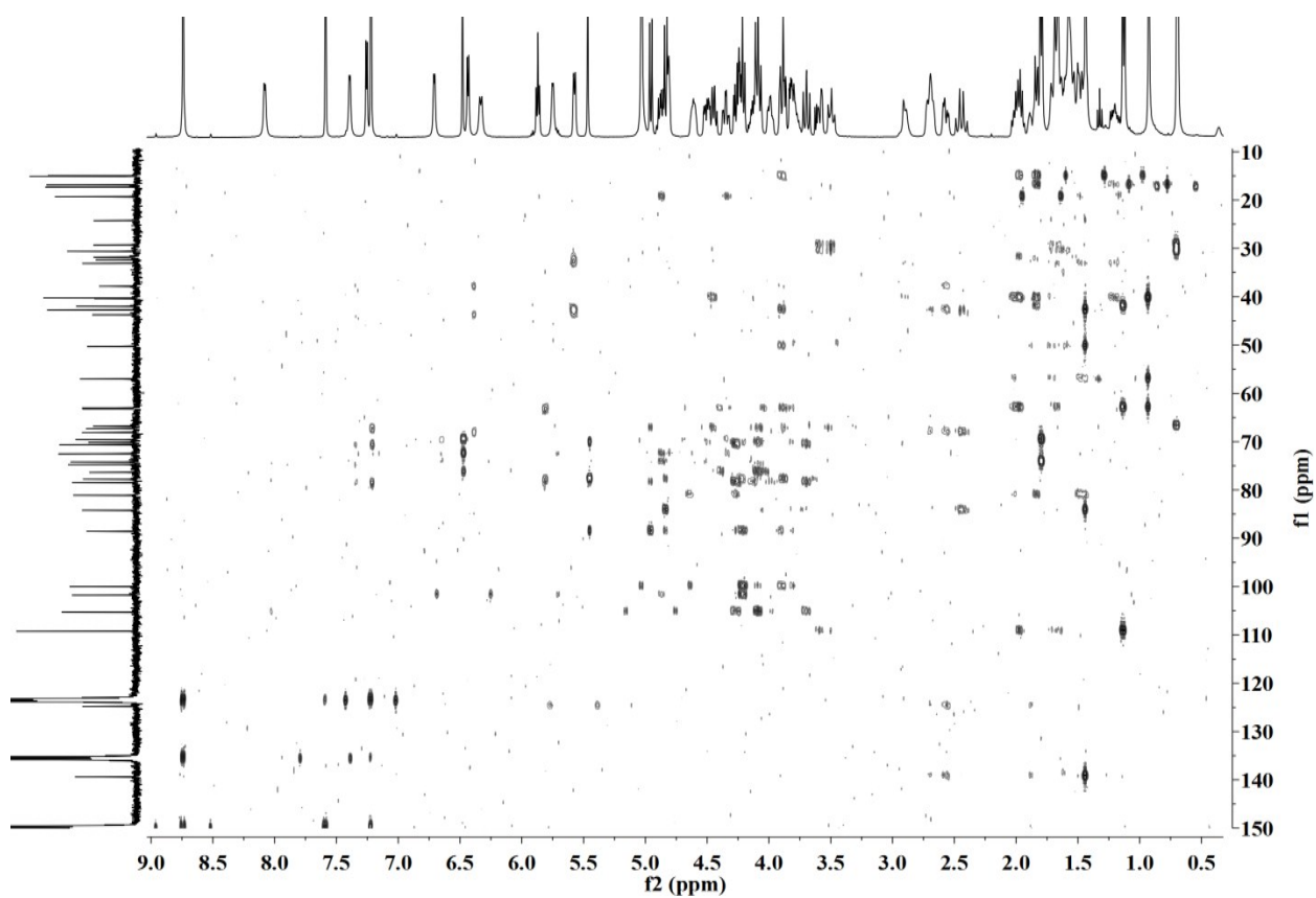
Figure S33. TOCSY NMR spectrum of compound 5 (pyridine- d_5 )
