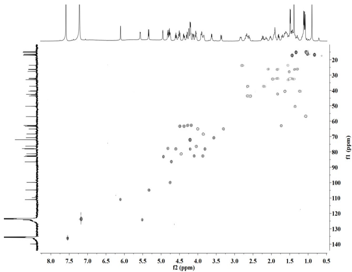
Figure S38. HSQC NMR spectrum of compound 6 (pyridine- d_5 )
