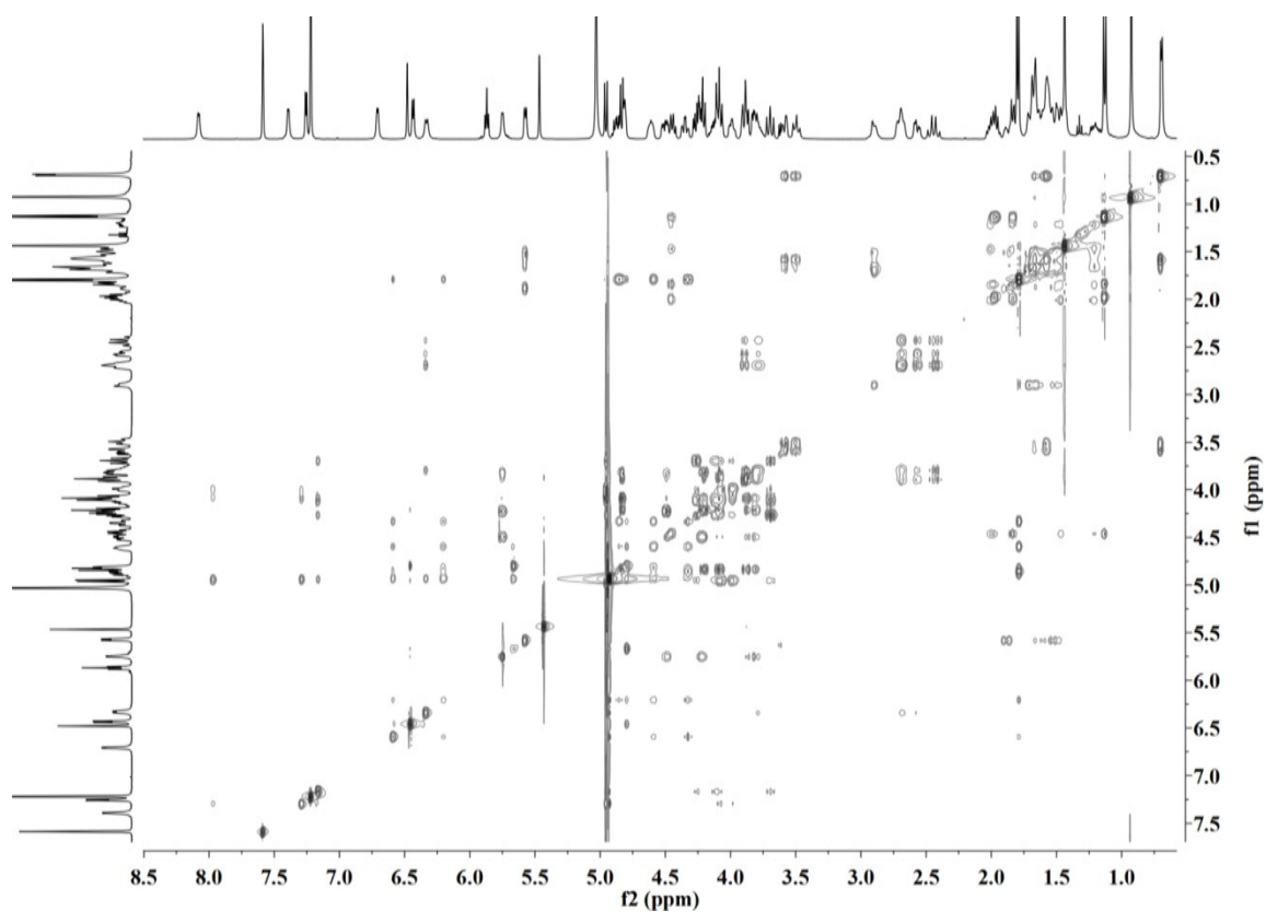
Figure S33. TOCSY NMR spectrum of compound 5 (pyridine- d_5 )
