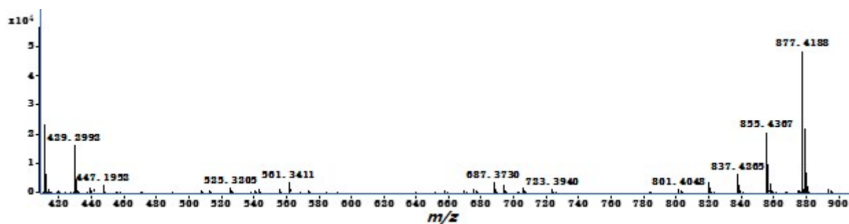
Figure S55. IR (KBr, disc) spectrum of compound 8
