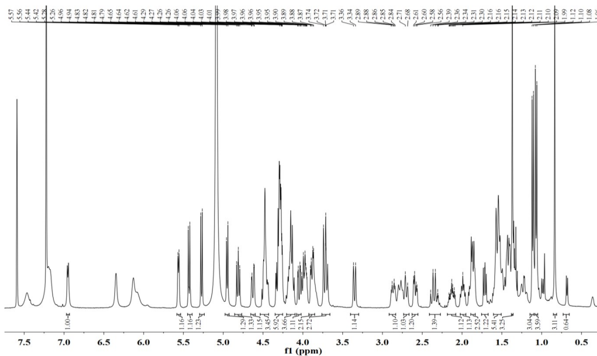
Figure S15. ^1\text{H} NMR spectrum of compound 3 (pyridine- d_5 )
