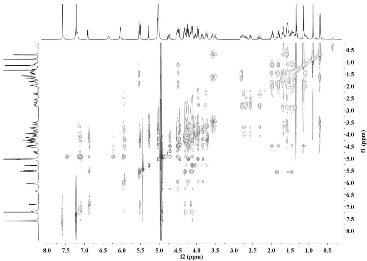
Figure S12. TOCSY NMR spectrum of compound 2 (pyridine- d 5 )
