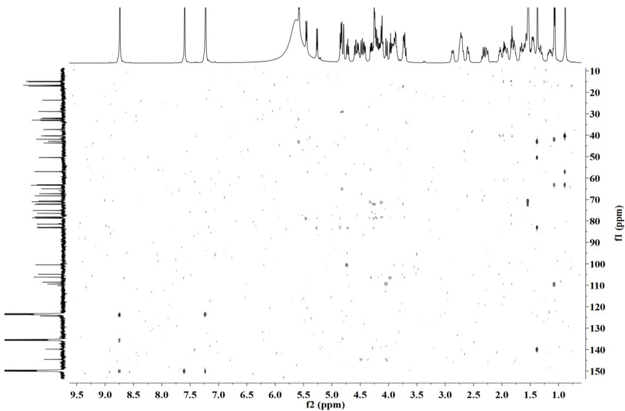
Figure S66. HMBC NMR spectrum of compound 10 (pyridine- d_5 )
