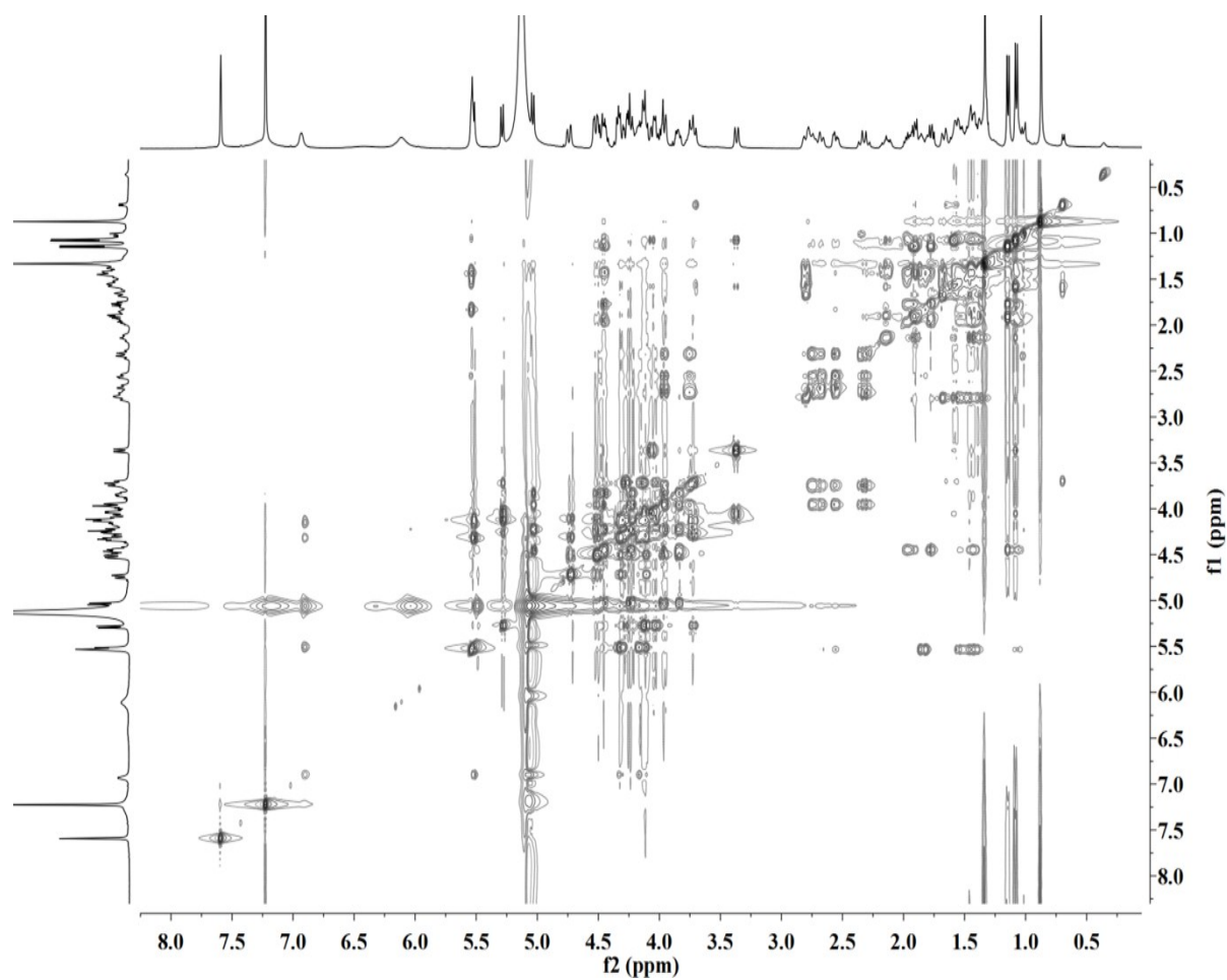
Figure S5. TOCSY NMR spectrum of compound 1 (pyridine- d_5 )
