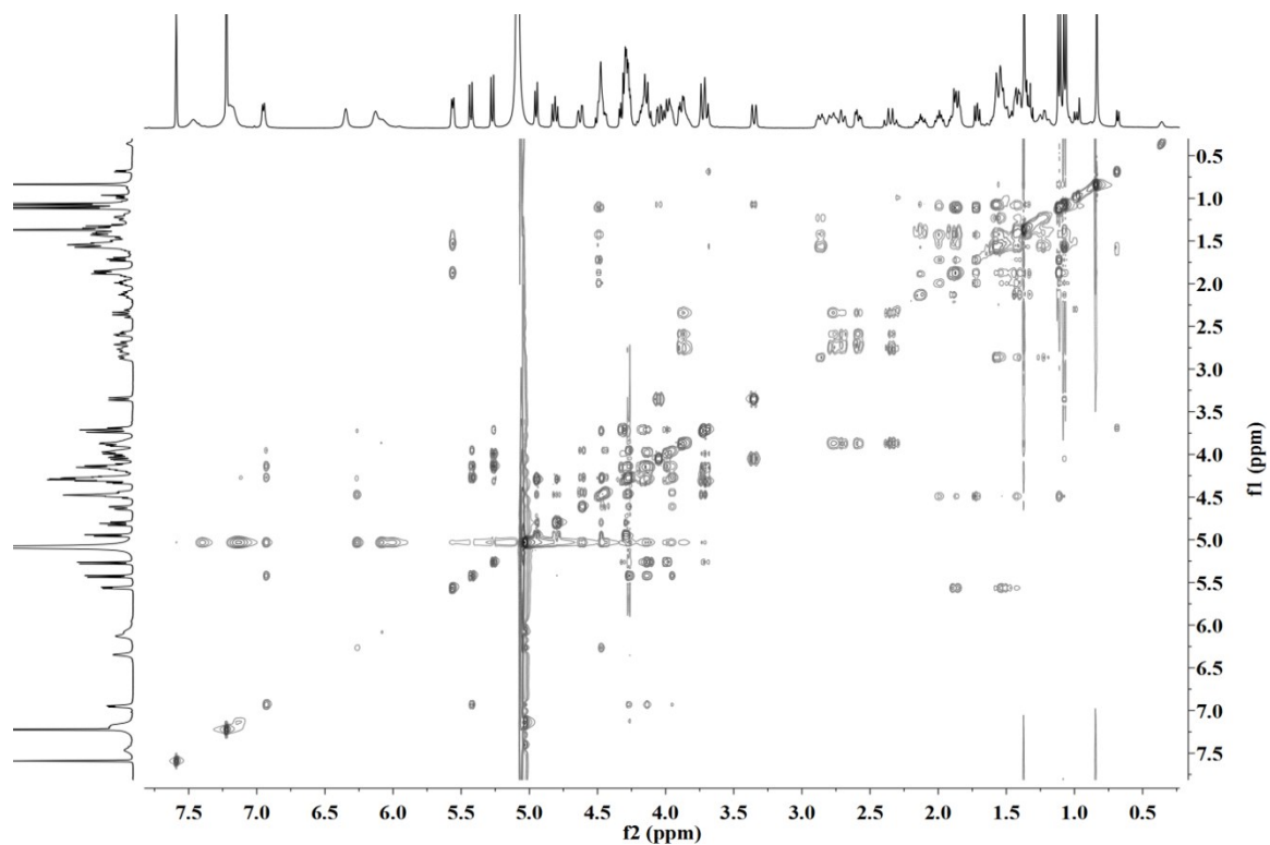
Figure S19. TOCSY NMR spectrum of compound 3 (pyridine- d_5 )
