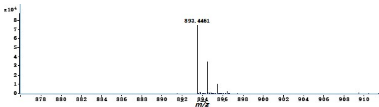
Figure S48. IR (KBr, disc) spectrum of compound 7
