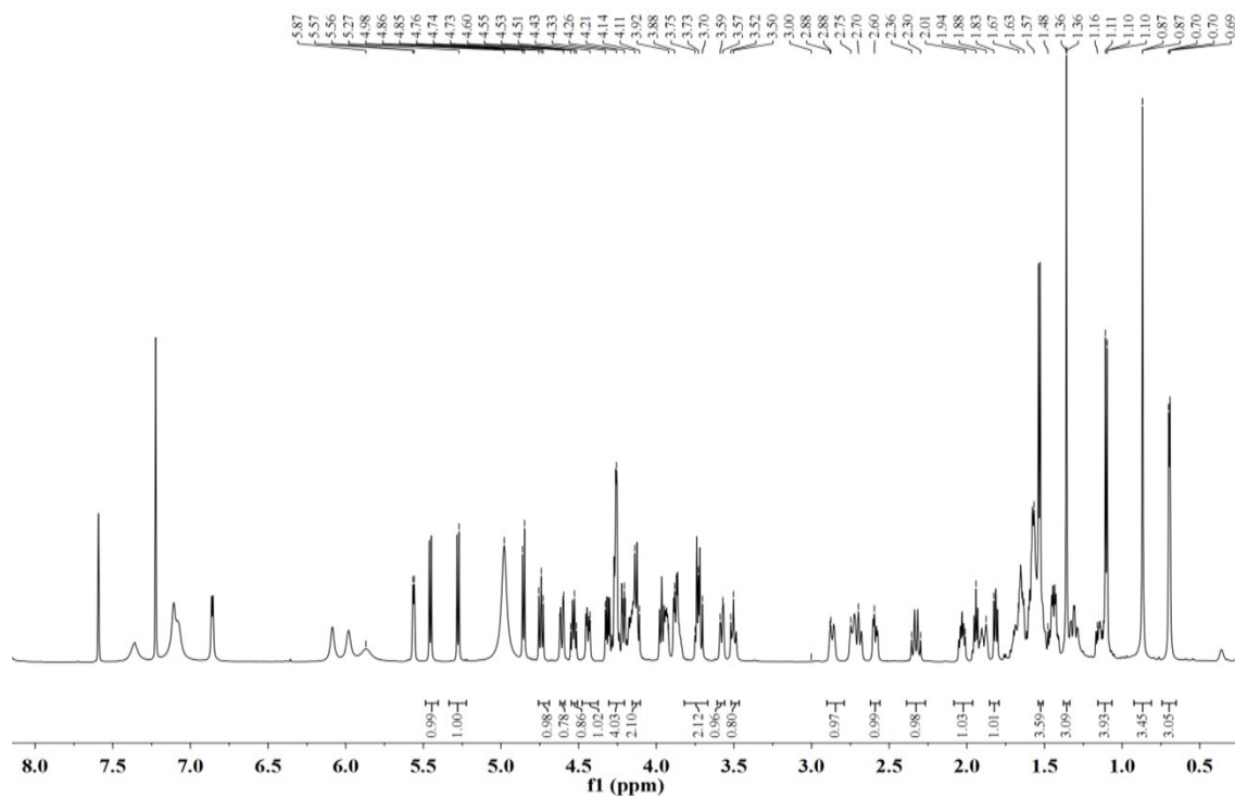
Figure S71. ^{13}\text{C} NMR spectrum of compound 11 (pyridine- d_5 )
