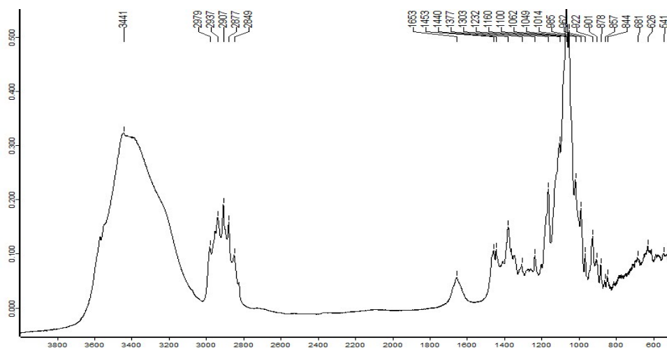
Figure S69. IR (KBr, disc) spectrum of compound 10
