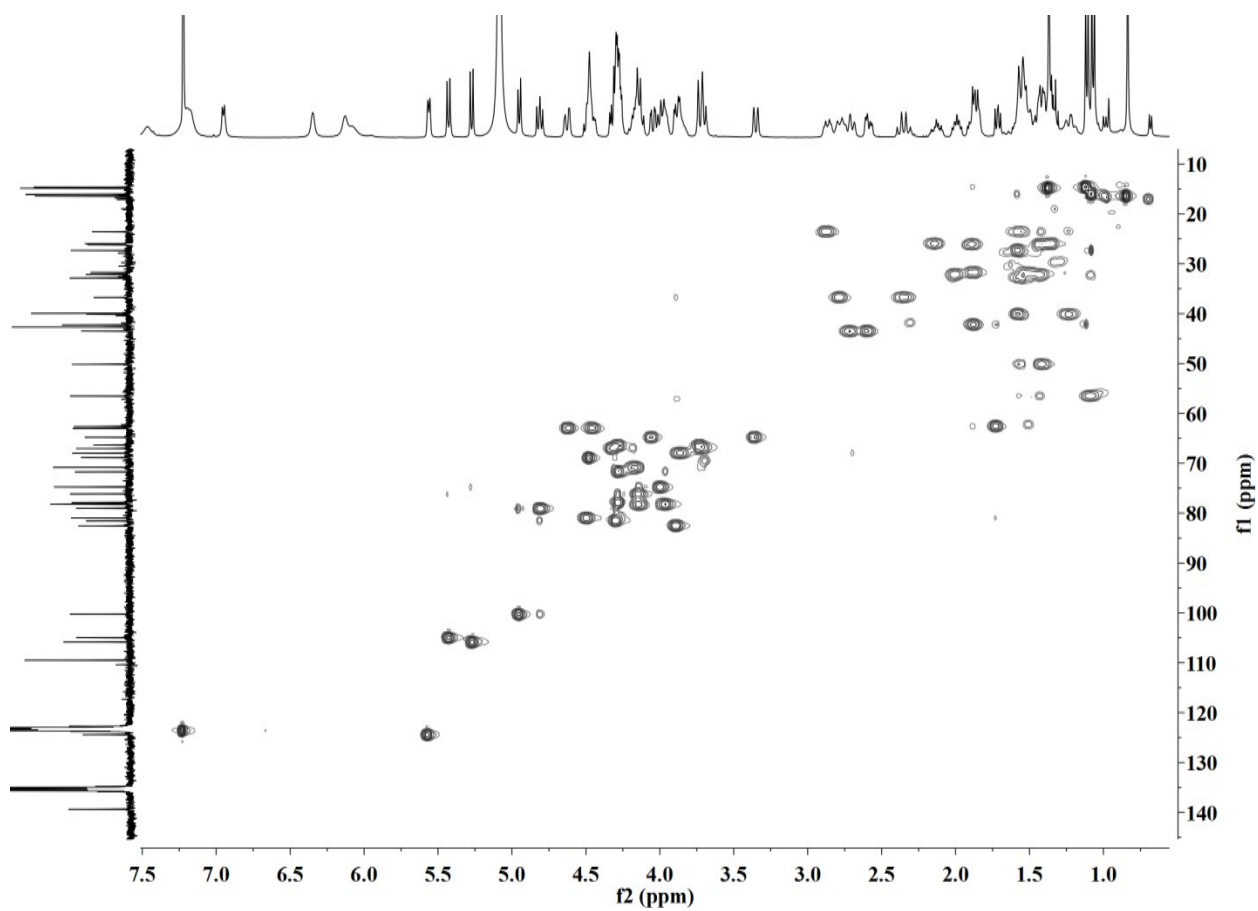
Figure S17. HSQC NMR spectrum of compound 3 (pyridine- d_5 )
