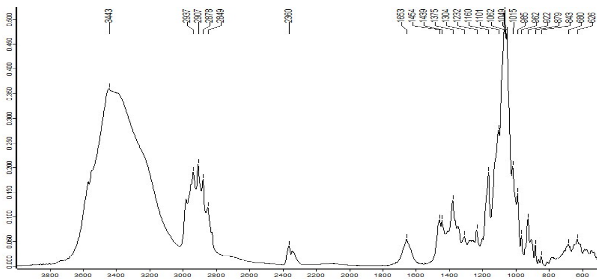
Figure S62. IR (KBr, disc) spectrum of compound 9
