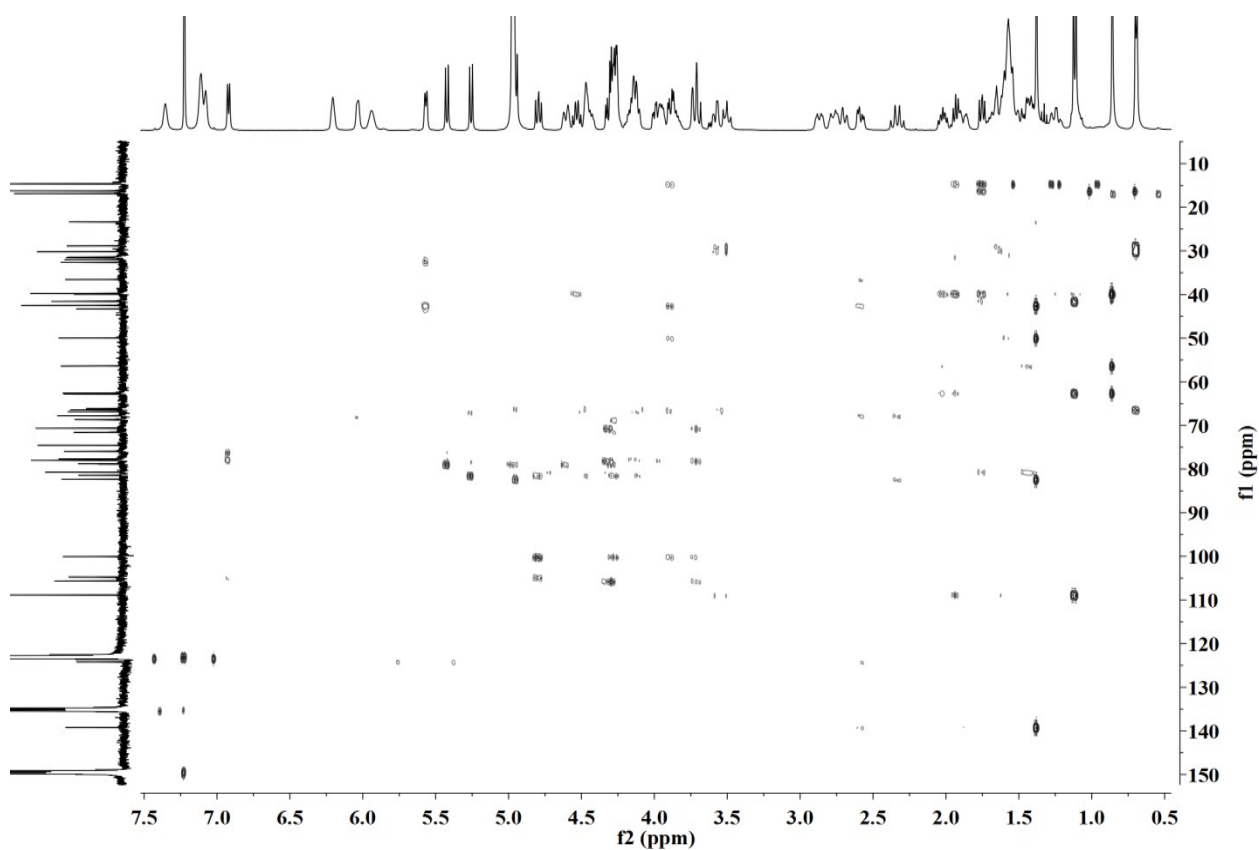
Figure S26. TOCSY NMR spectrum of compound 4 (pyridine- d_5 )
