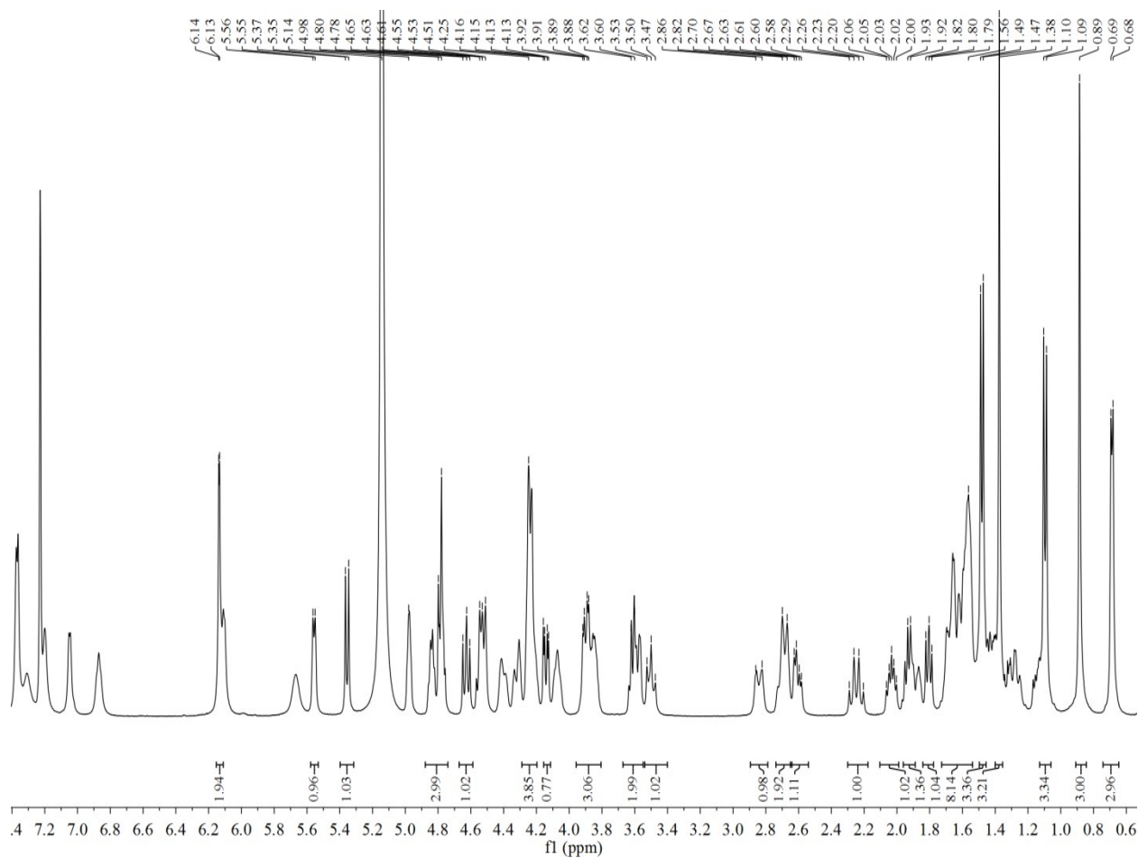
Figure S43. ^{13}\text{C} NMR spectrum of compound 7 (pyridine- d_5 )
