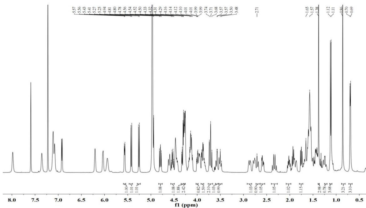
Figure S22. ^1\text{H} NMR spectrum of compound 4 (pyridine- d_5 )
