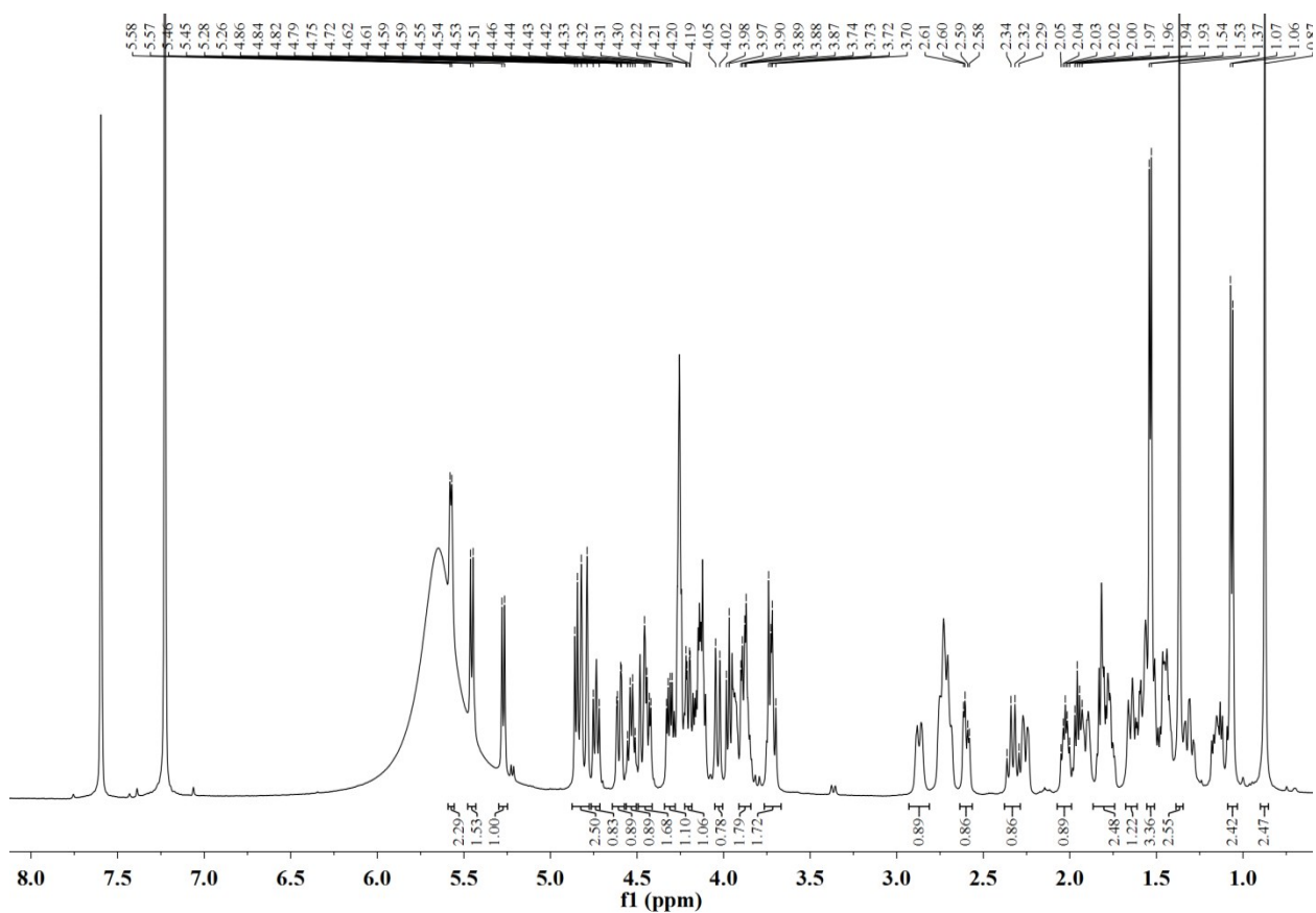
Figure S63. ^1\text{H} NMR spectrum of compound 10 (pyridine- d_5 )
