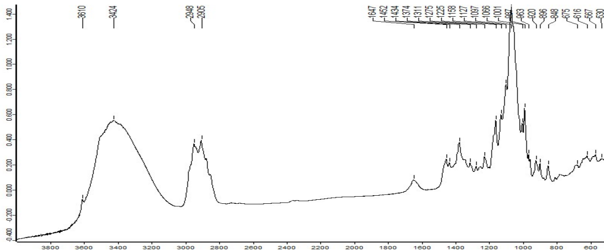
Figure S41. IR (KBr, disc) spectrum of compound 6
