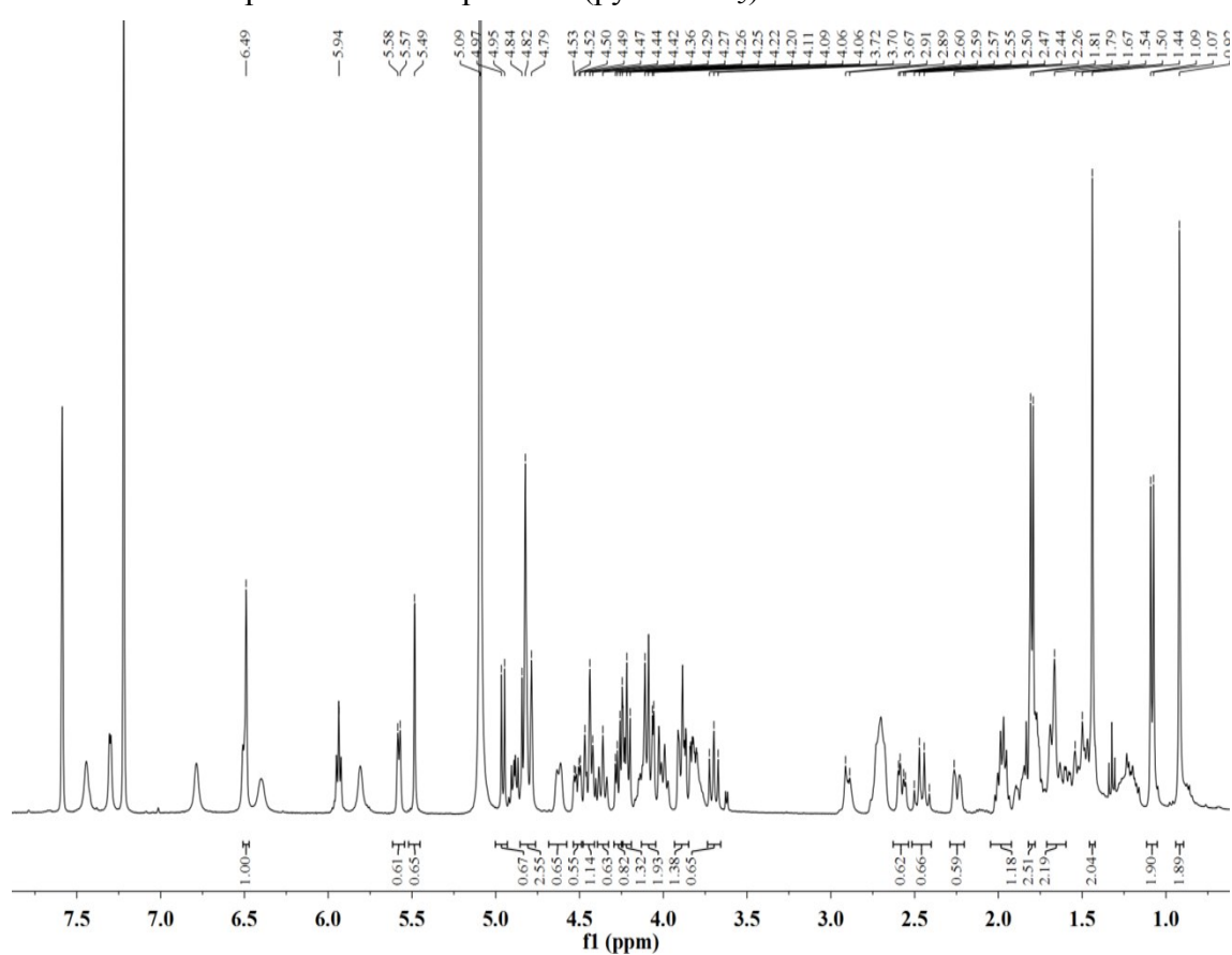
Figure S57. ^{13}\text{C} NMR spectrum of compound 9 (pyridine- d_5 )
