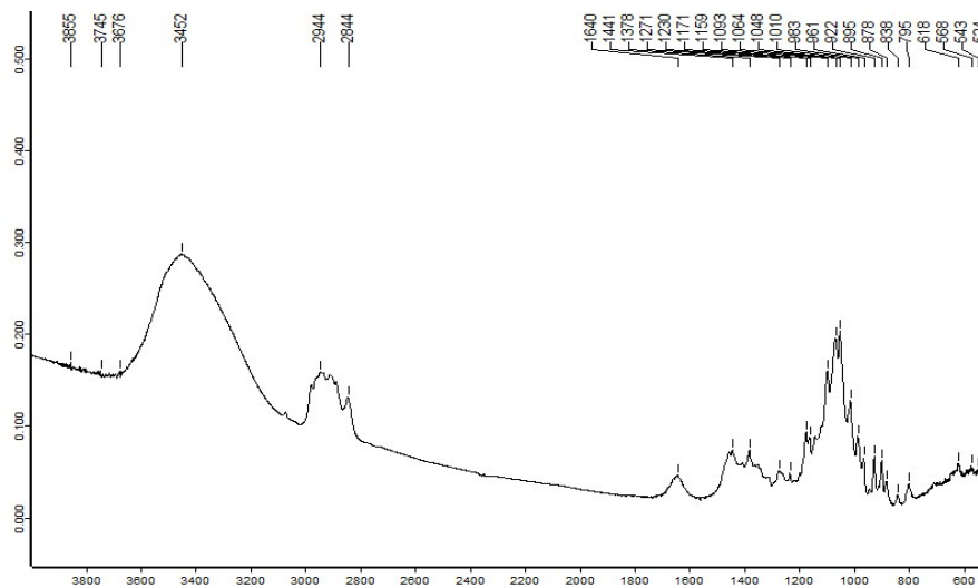
Figure S55. IR (KBr, disc) spectrum of compound 8
