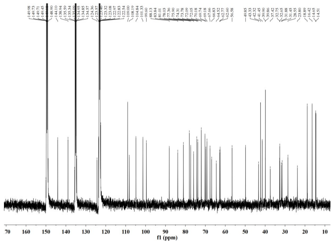
Figure S57. ^{13}\text{C} NMR spectrum of compound 9 (pyridine- d_5 )
