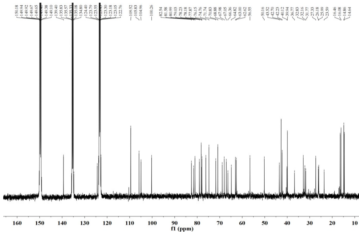
Figure S17. HSQC NMR spectrum of compound 3 (pyridine- d_5 )
