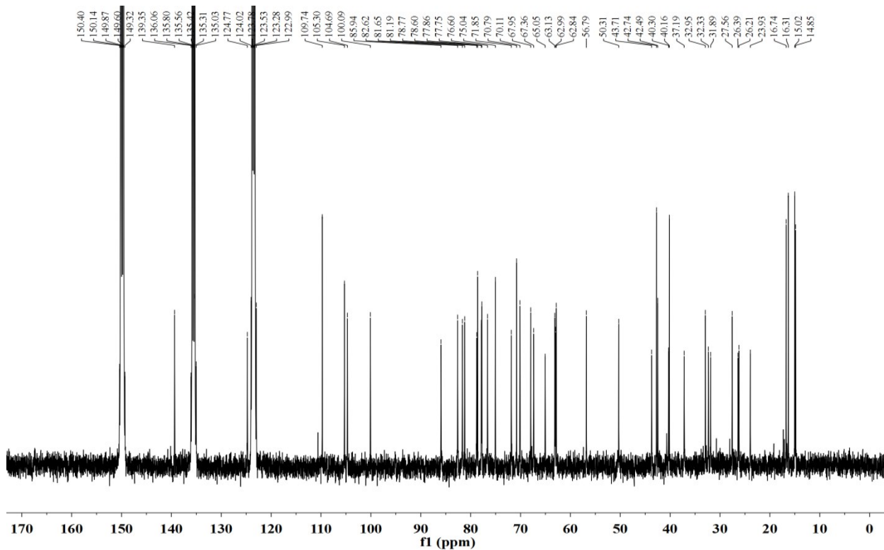
Figure S2. ^{13}\text{C} NMR spectrum of compound 1 (pyridine- d_5 )
