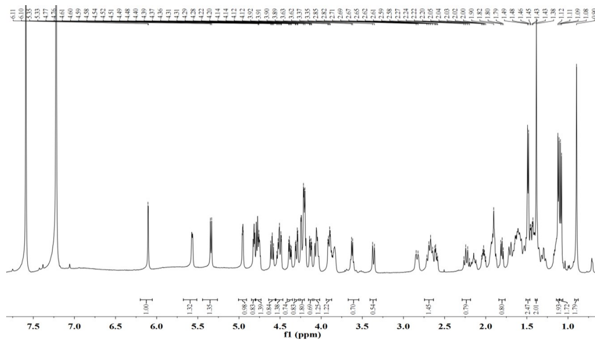
Figure S36. ^1\text{H} NMR spectrum of compound 6 (pyridine- d_5 )
