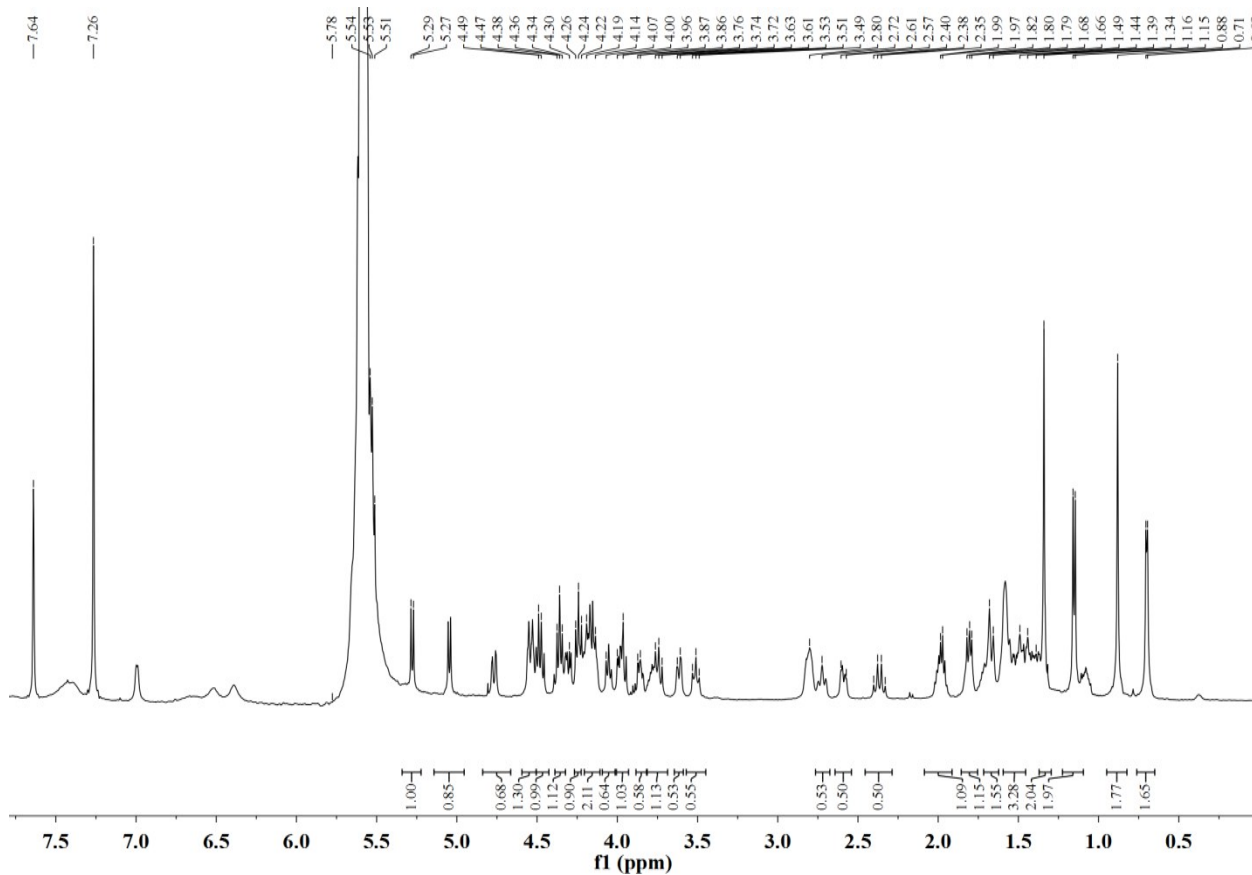
Figure S8. 1 H NMR spectrum of compound 2 (pyridine- d 5 )
