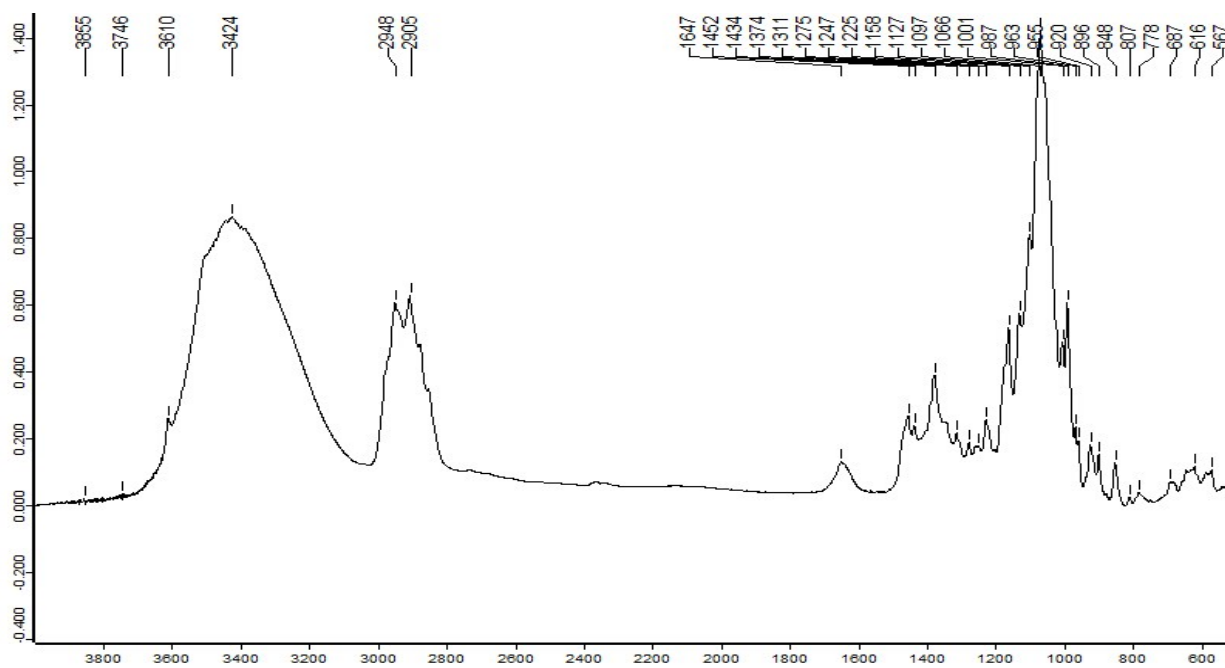
Figure S7. IR (KBr, disc) spectrum of compound 1
