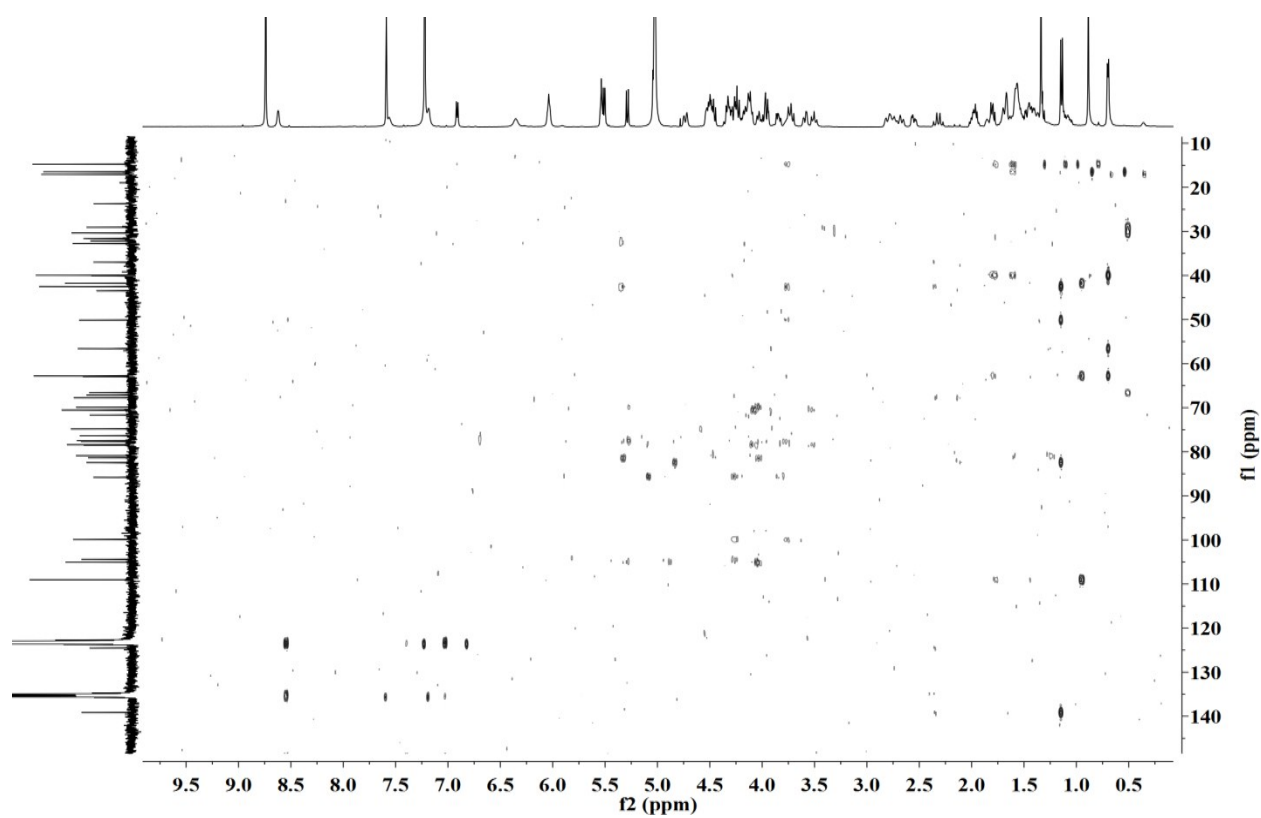
Figure S12. TOCSY NMR spectrum of compound 2 (pyridine- d 5 )
