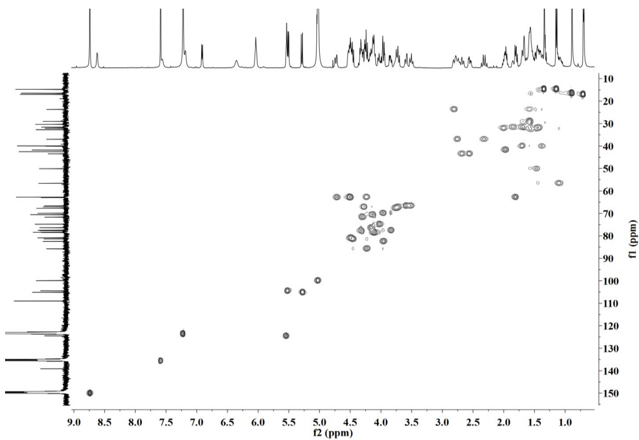
Figure S10. HSQC NMR spectrum of compound 2 (pyridine- d_5 )
