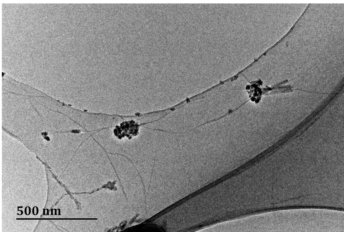
Figure 4 The TEM image of Co 9 S 8 /RGO-CNT
