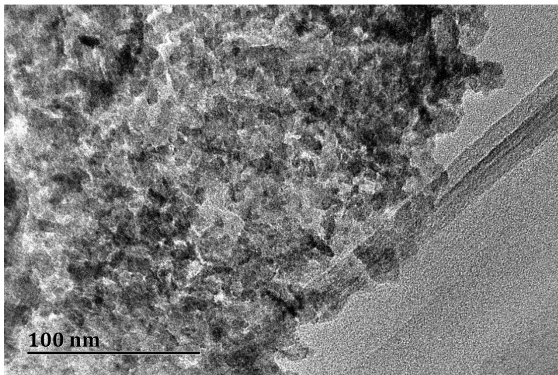
Figure 2 The TEM image of Co 9 S 8 /RGO
