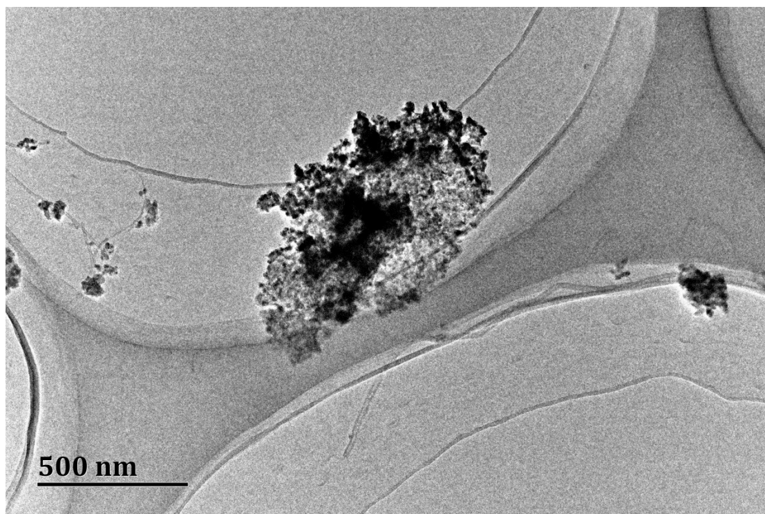
Figure 1 The TEM image of Co 9 S 8 /RGO
