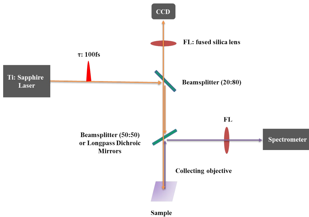
Figure S1. Experimental setup for measuring SH spectra.
