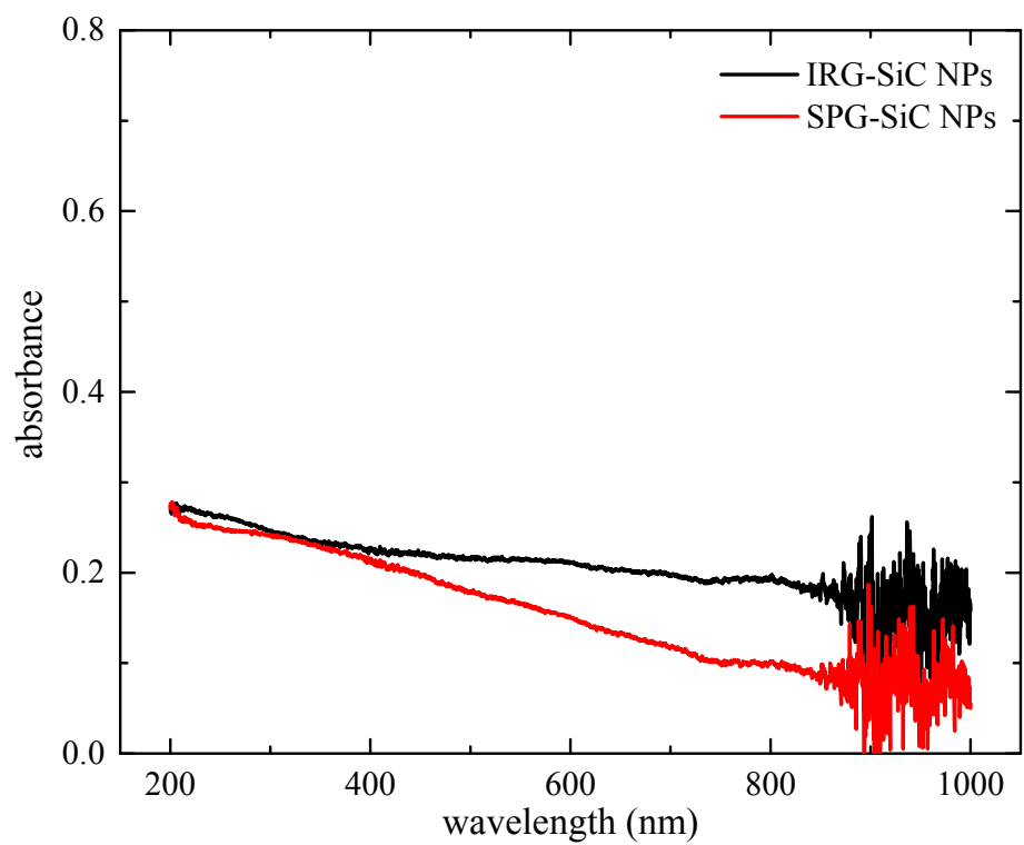
Figure S2. Ultraviolet-visible (UV3150, Shimadzu, Japan) absorption spectrum of SiC NPs dispersed in deionized water (0.05mg / ml).
