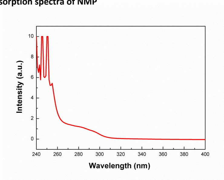
Fig. S1 The UV-vis absorption spectra of NMP. Basically, there is no absorption for NMP at the wavelength of 365 nm.
