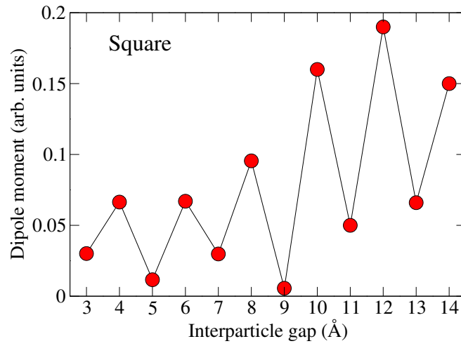
Figure S1: dipole moment evolution in the square arrangement as a function of the interparticle gaps.
