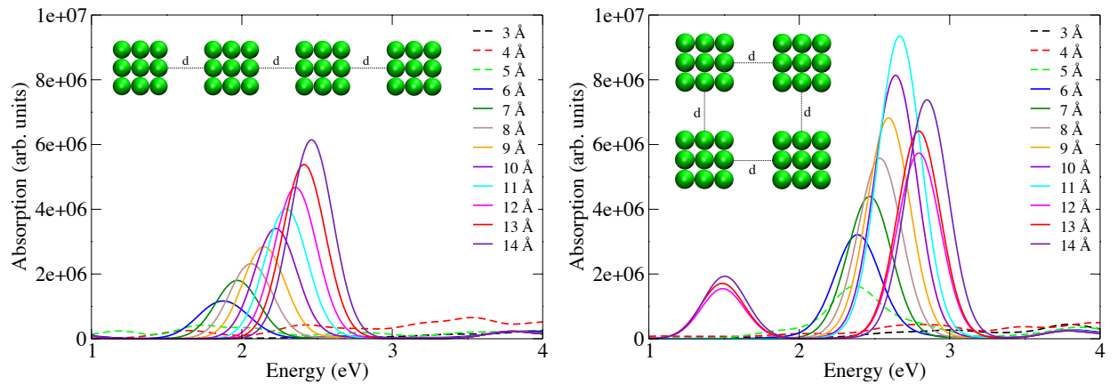
Figure S2: absorption spectrum of cube shaped Al nanoparticle arrangements.
