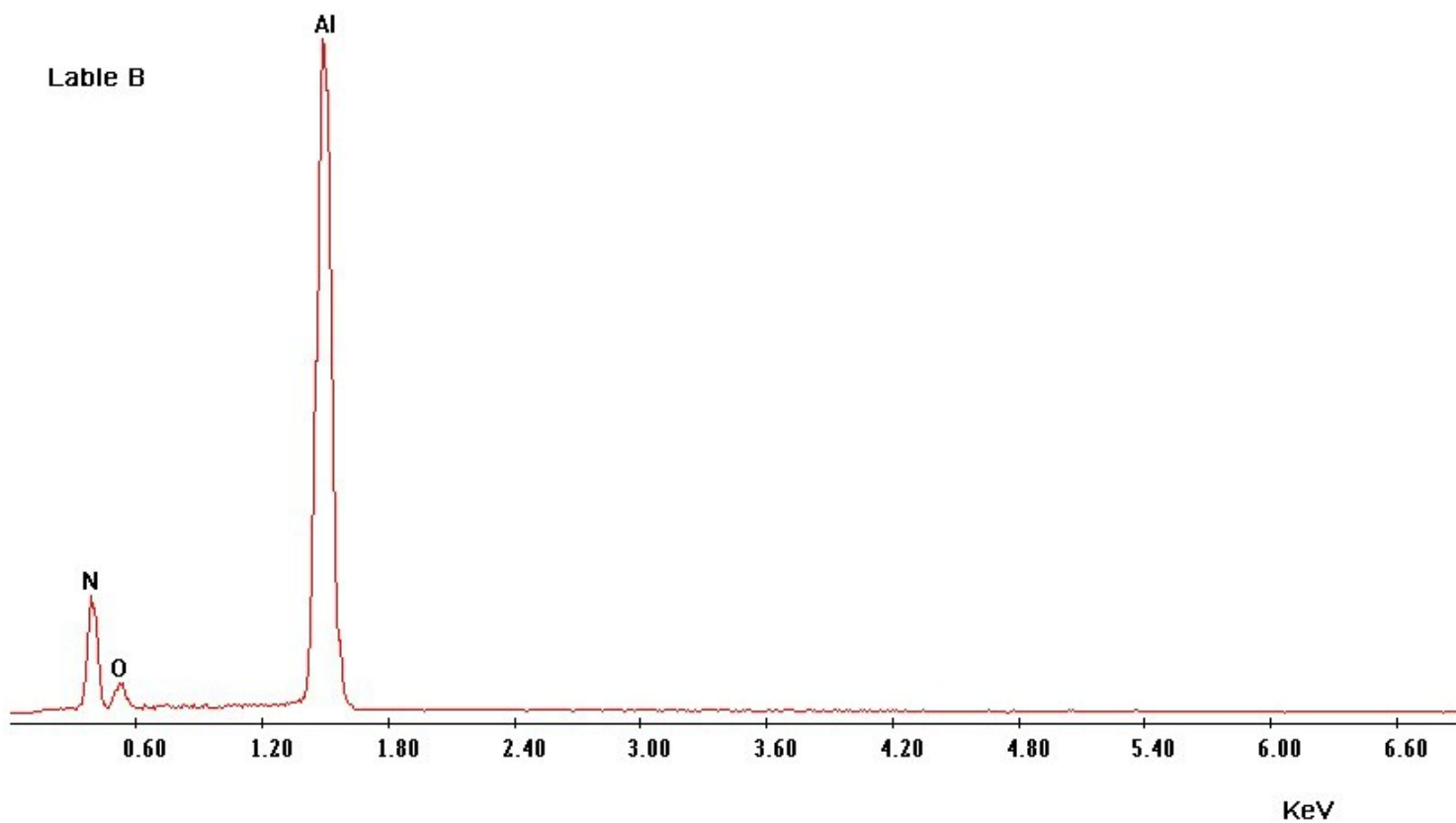
The EDS spectra from the AlN nanocones under the NH 3 flow of (A) 10 sccm, (B) 100 sccm at 950 °C.
