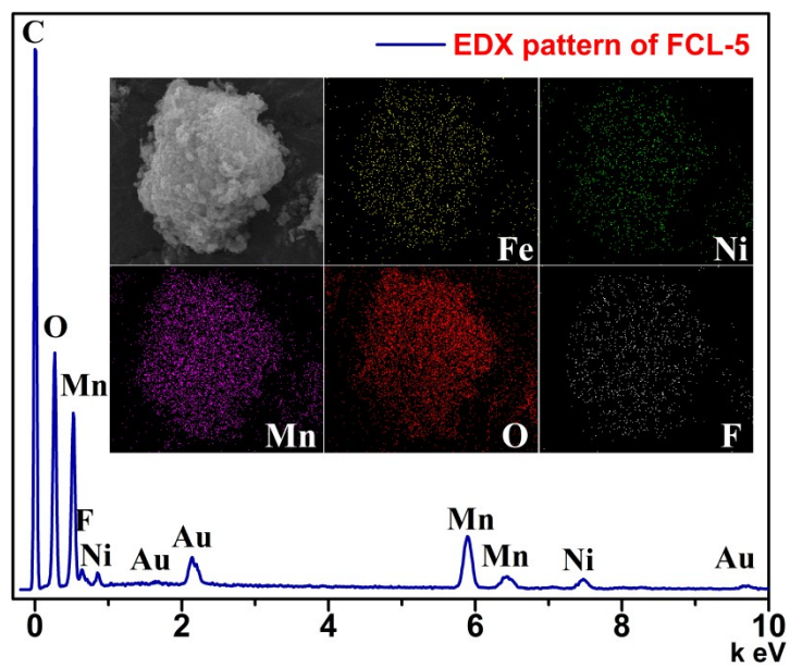
Fig. S2 EDX pattern and the element mappings of FCL-5.
