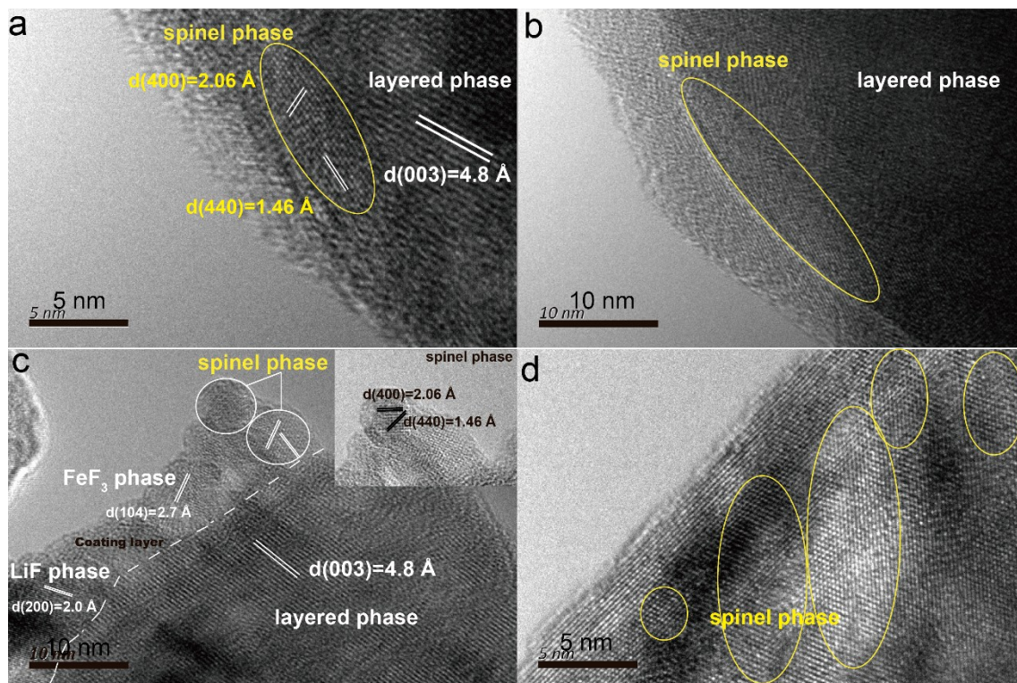
Fig. S1 HRTEM images of (a) FCL-5, (b) FCL-7, and (c, d) FCL-10 in different areas.
