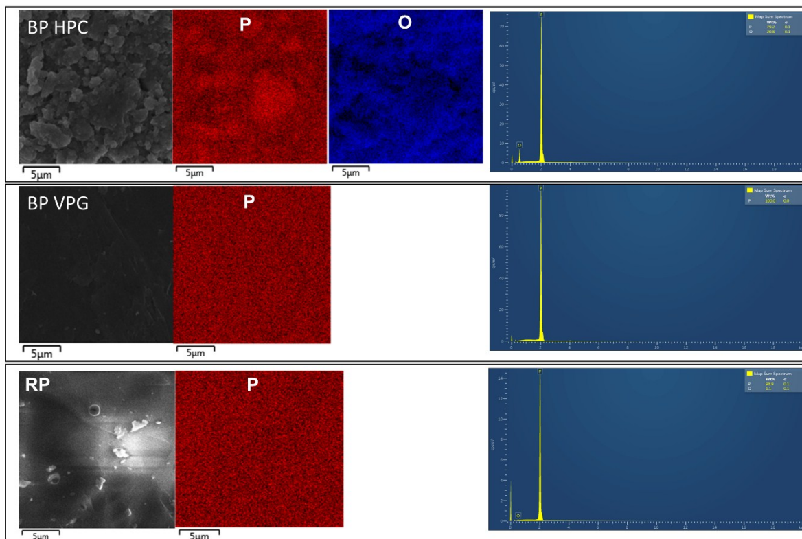
Figure S1. SEM-EDX mapping and energy-dispersive X-ray (EDX) spectroscopy of BP HPC, BP VPG and commercial RP.
