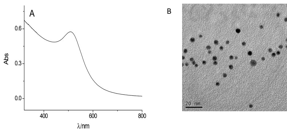
Figure S1 UV-vis absorption spectrum (A) and TEM image (B) of Au NPs.
