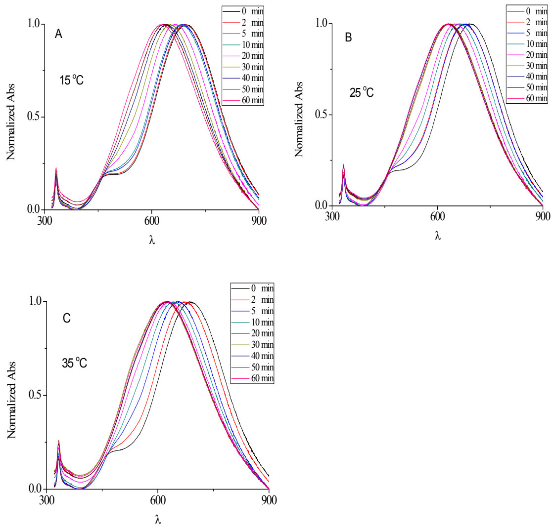
Fig. S5 UV-vis absorption spectra of different etching times and temperature.
