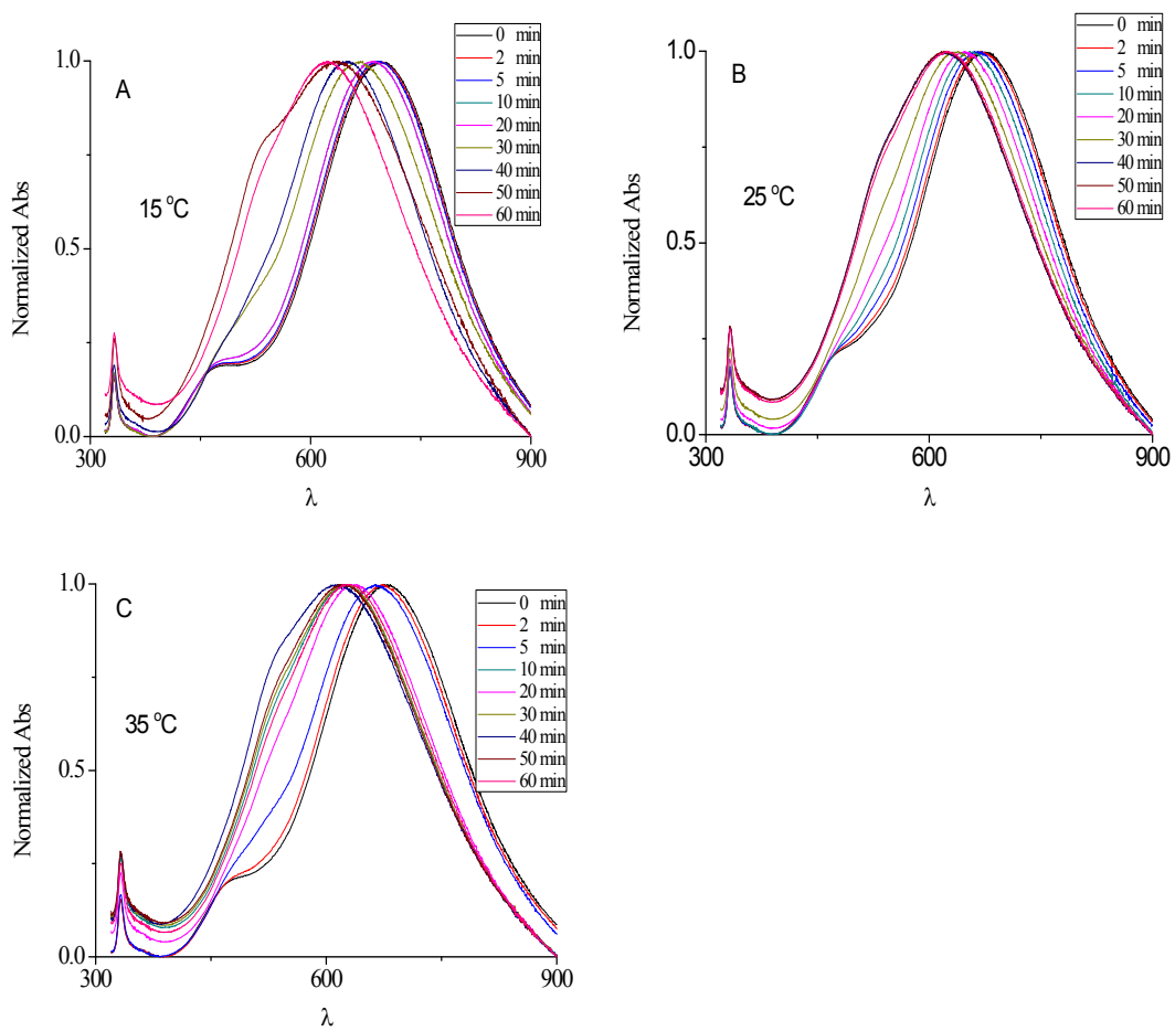
Fig. S4 UV-vis absorption spectra of different catalytic times and temperatures.
