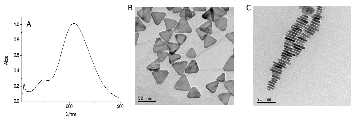
Figure S2 UV-vis absorption spectrum (A) and TEM image (B and C) of Ag TNPs.
