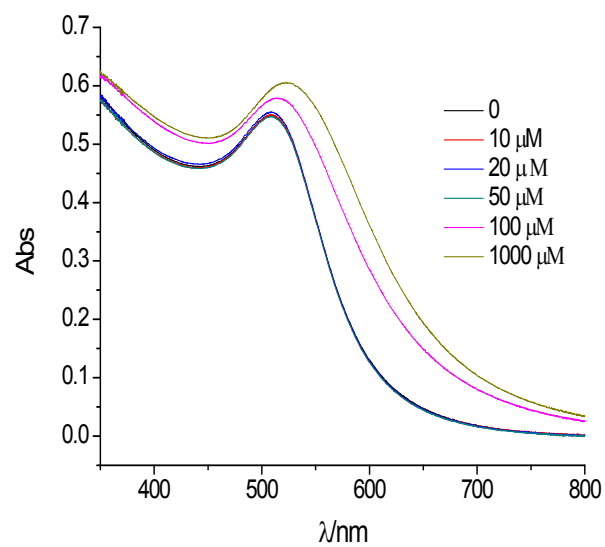
Fig. S3 UV-vis absorption spectra of Au NPs before and after addition of different concentration of Cys.
