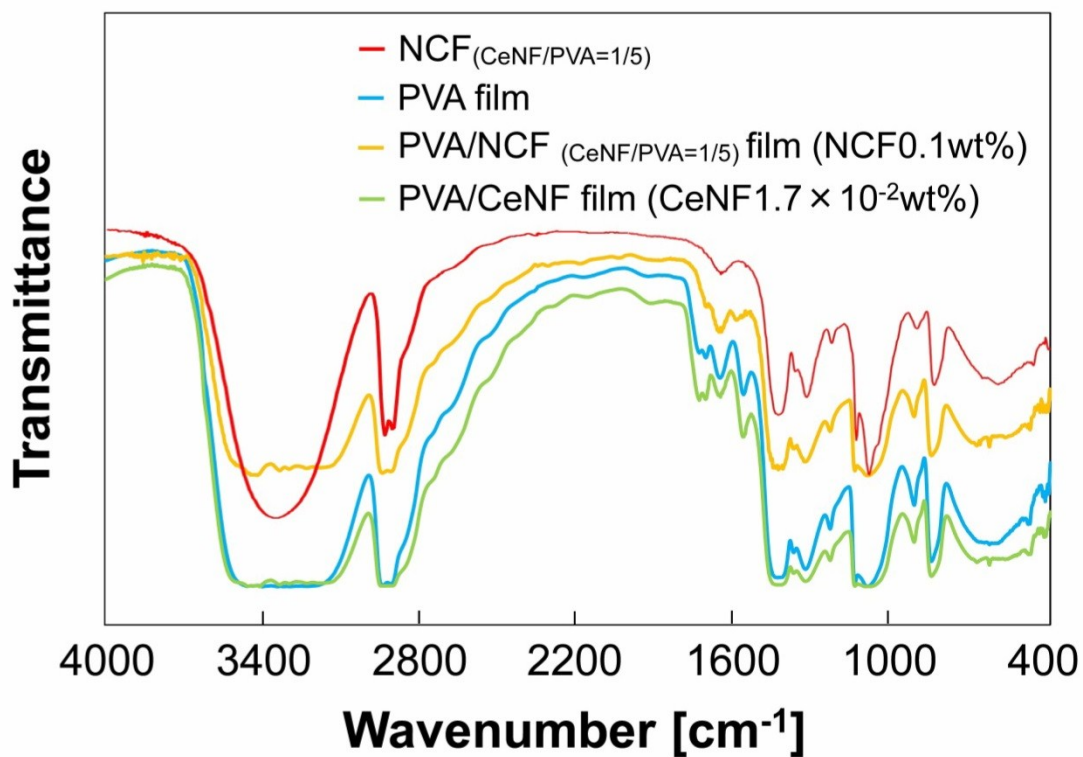
Fig.S2 FTIR spectra of NCF film, PVA film, NCF/PVA composite film and CeNF/PVA composite film.
