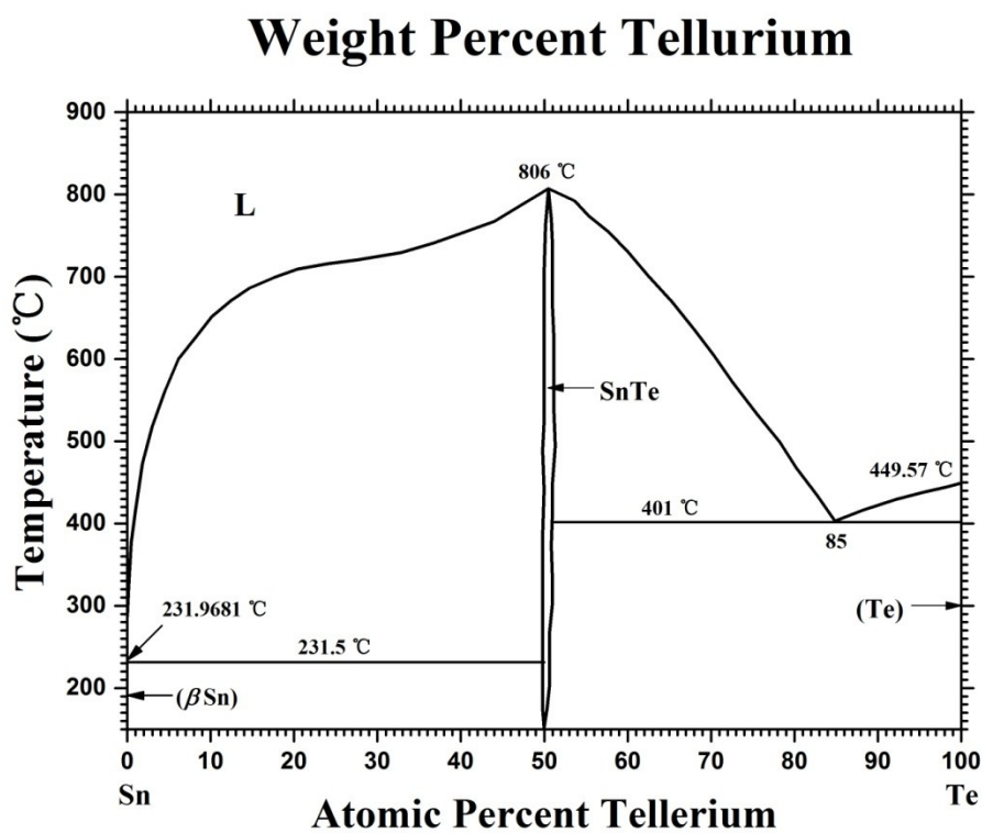
Fig. S1 Binary Sn-Te phase diagram.
