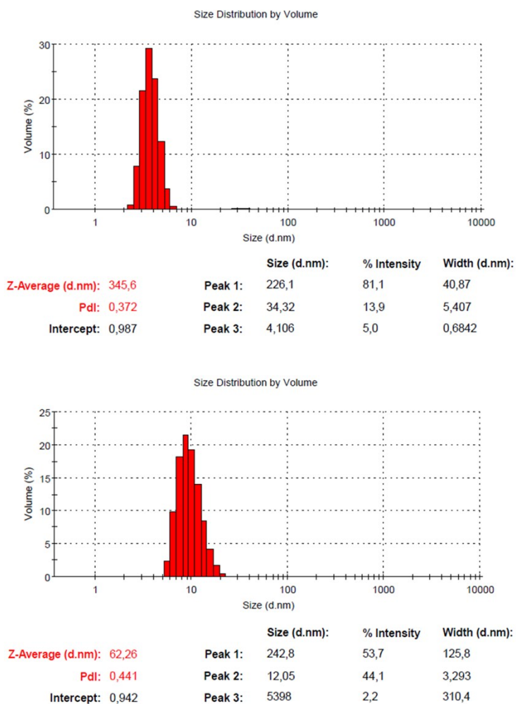
Fig. S1. DLS size determination of CdS QDs. DLS measurements were conducted on blue-green (top) and orange-red (bottom) solutions. Results are informed as volume (%) versus size (nm). Z-average size and polydispersity Index (PDI) are informed at the bottom each image.
