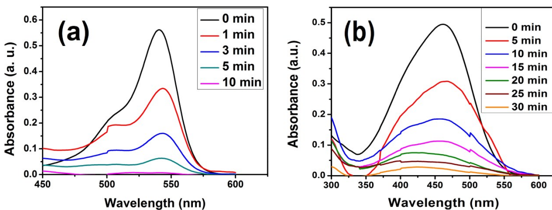
Figure SI-1. UV-vis absorption spectral changes of (a) RB and (b) MO dye in presence of PC2 due to visible light irradiated photo catalysis
