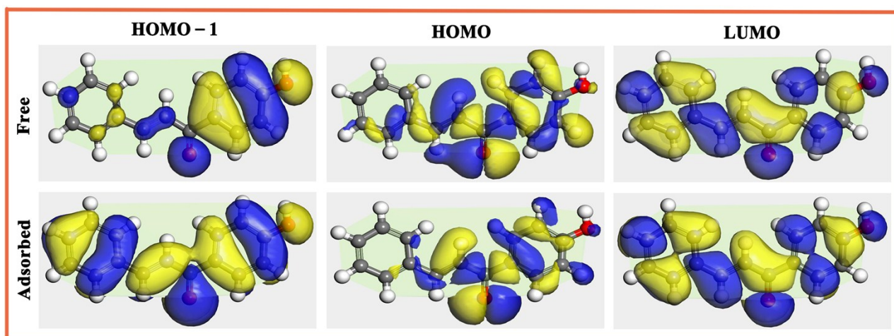
Fig. S3 Molecular orbital plots for the Inh1 molecule from the HOMO-1 to LUMO under the free (upper row) and adsorbed state (lower row).
