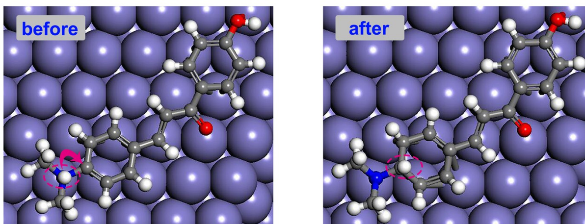
Fig. S1 Adsorption configurations of Inh3H before and after the geometry optimization.
