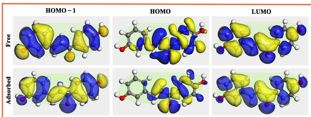
Fig. S2 Molecular orbital plots for the Inh2 molecule from the HOMO-1 to LUMO under the free (upper row) and adsorbed state (lower row).
