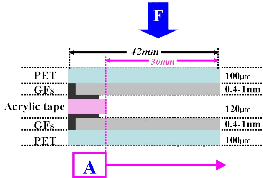
Figure S3. A schematic cross-sectional view of the device
