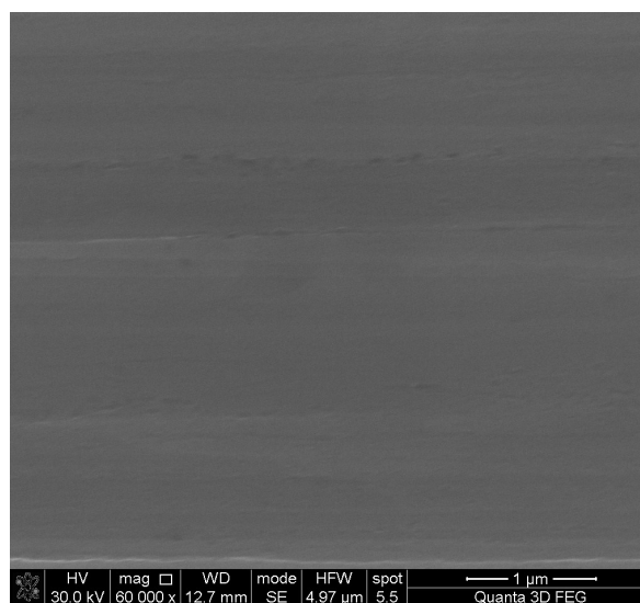
Figure S2. FESEM image of the graphene film on the copper foil substrate
