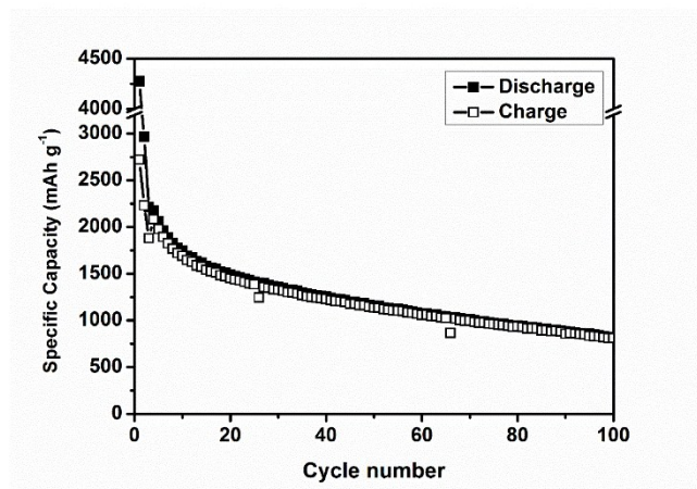
Fig.S3 Cyclic performance of Si@SiO x particles, with 0.1A g -1 current density.
