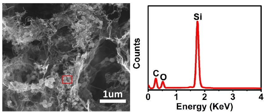
Fig.S2 EDS spectra of Si@SiO x /CNTs/GA-1 composite.
